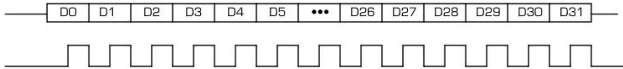
FIGURE 3 PMC BISERIAL-III-OSEH TIMING DIAGRAM
