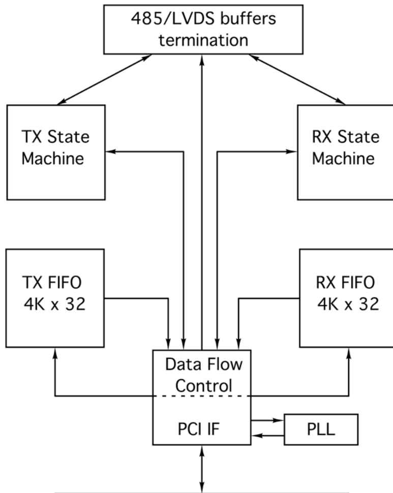
PMC-BISERIAL-III-OSEH BLOCK DIAGRAM
