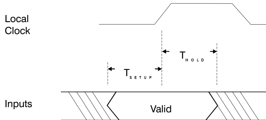
Figure 7-1. PCI 9052 Local Output Delay
