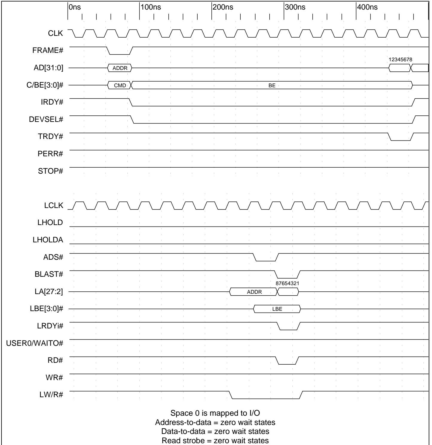
Timing Diagram 9-32. Direct Slave Single Read from 32 Bit Local Bus Big Endian and Multiplexed Local Bus (J Mode)
