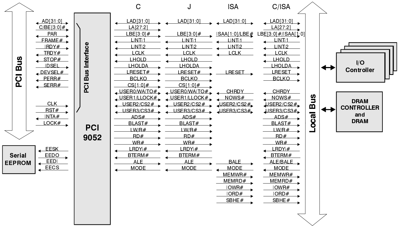
Figure 8-2. Typical Bus Target Interface Adapter (C, J, ISA, and C/ISA Modes)
