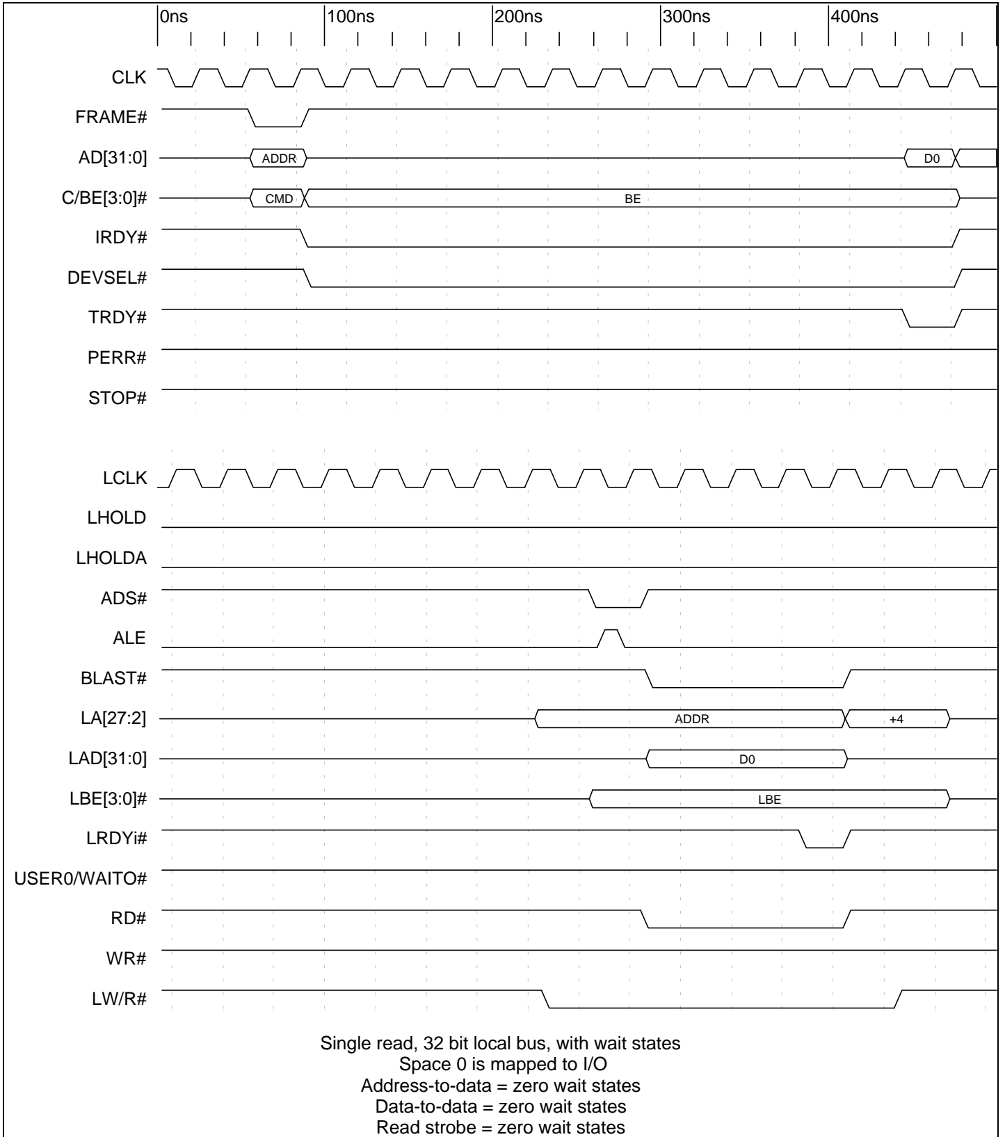
Timing Diagram 9-10. Direct Slave Single Read with Wait States (32 Bit Local Bus)
