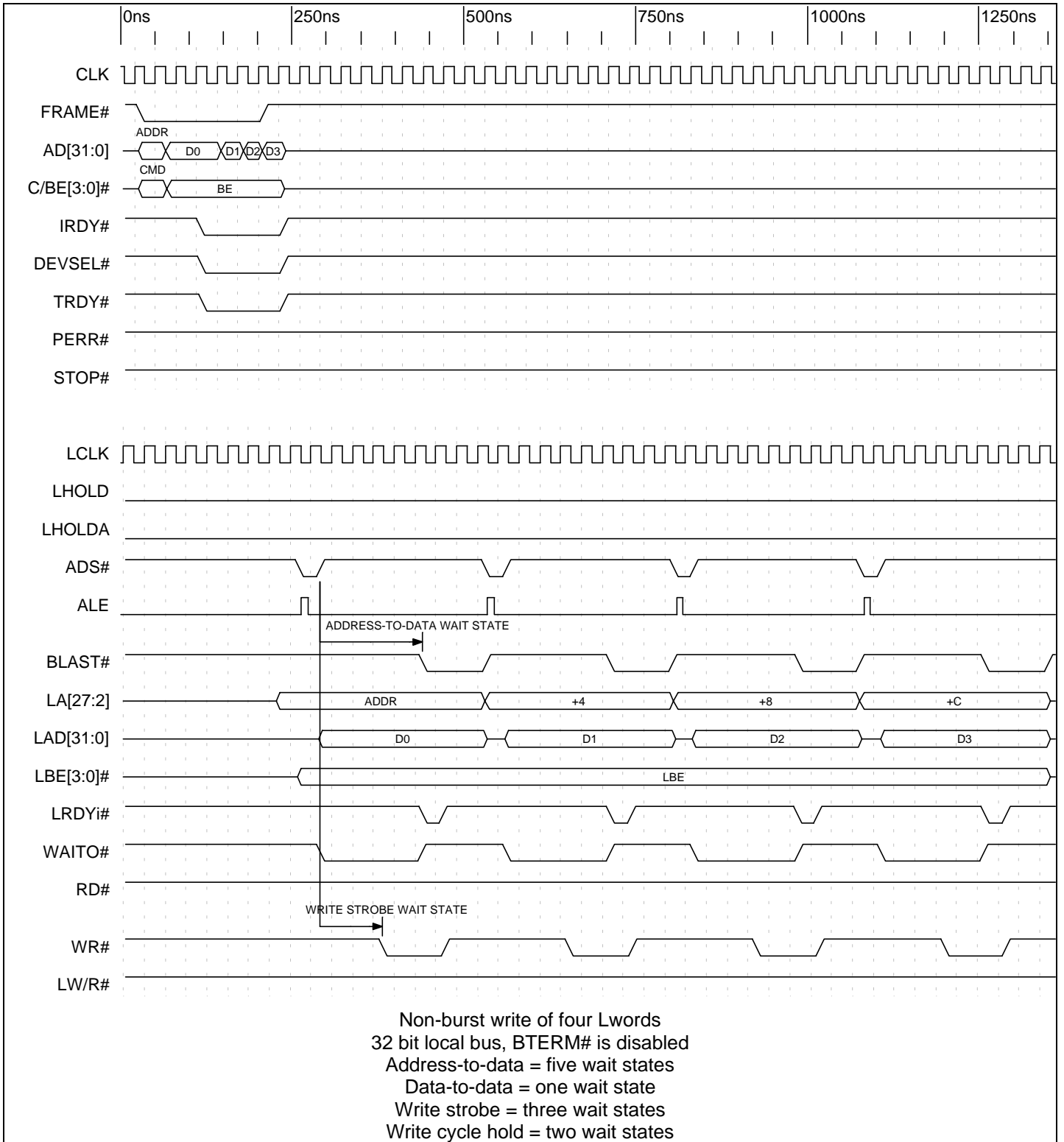
Timing Diagram 9-11. Direct Slave Non-Burst Write with Wait States (32 Bit Local Bus)
