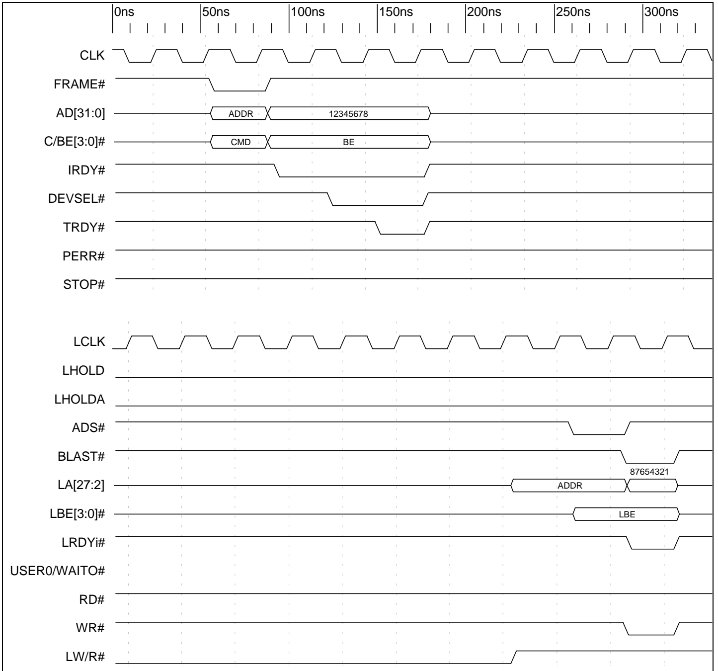
Timing Diagram 9-31. Direct Slave Single Write to 32 Bit Local Bus Big Endian and Multiplexed Local Bus (J Mode)
