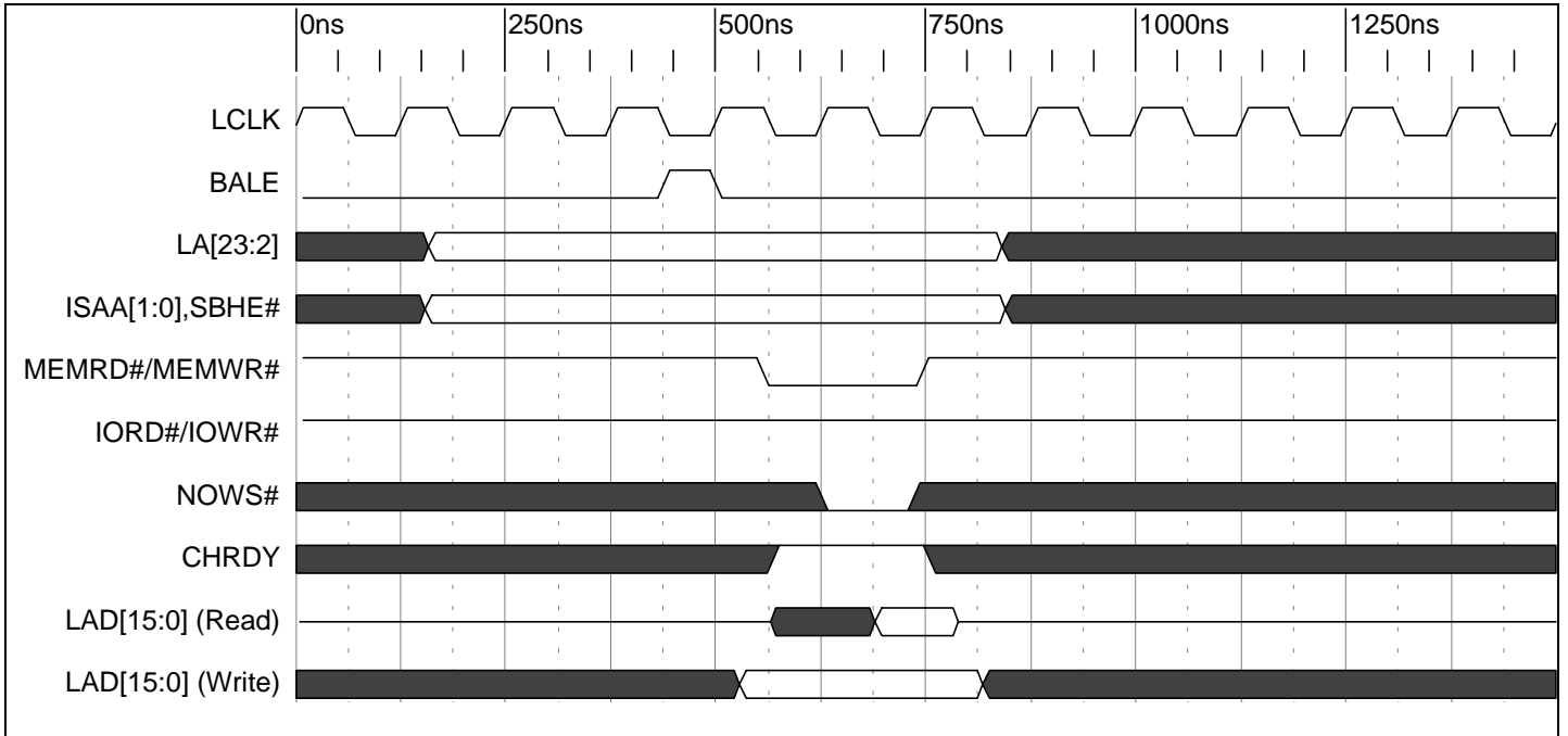
Timing Diagram 9-39. 8 Bit Memory Read/Write Compressed ISA Cycle (3 LCLK Shown)
