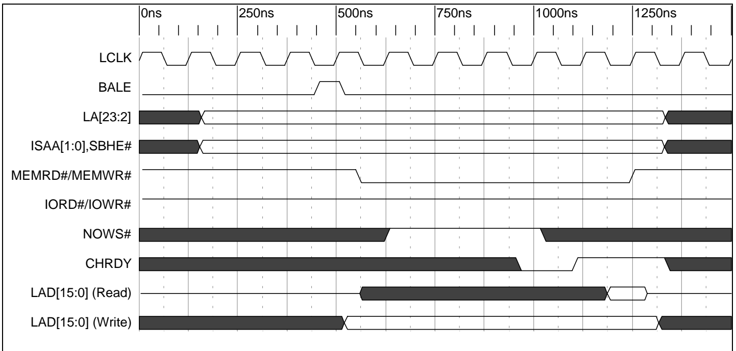
Timing Diagram 9-38. 8 Bit Memory Read/Write Extended ISA Cycle (7 LCLK Shown)
