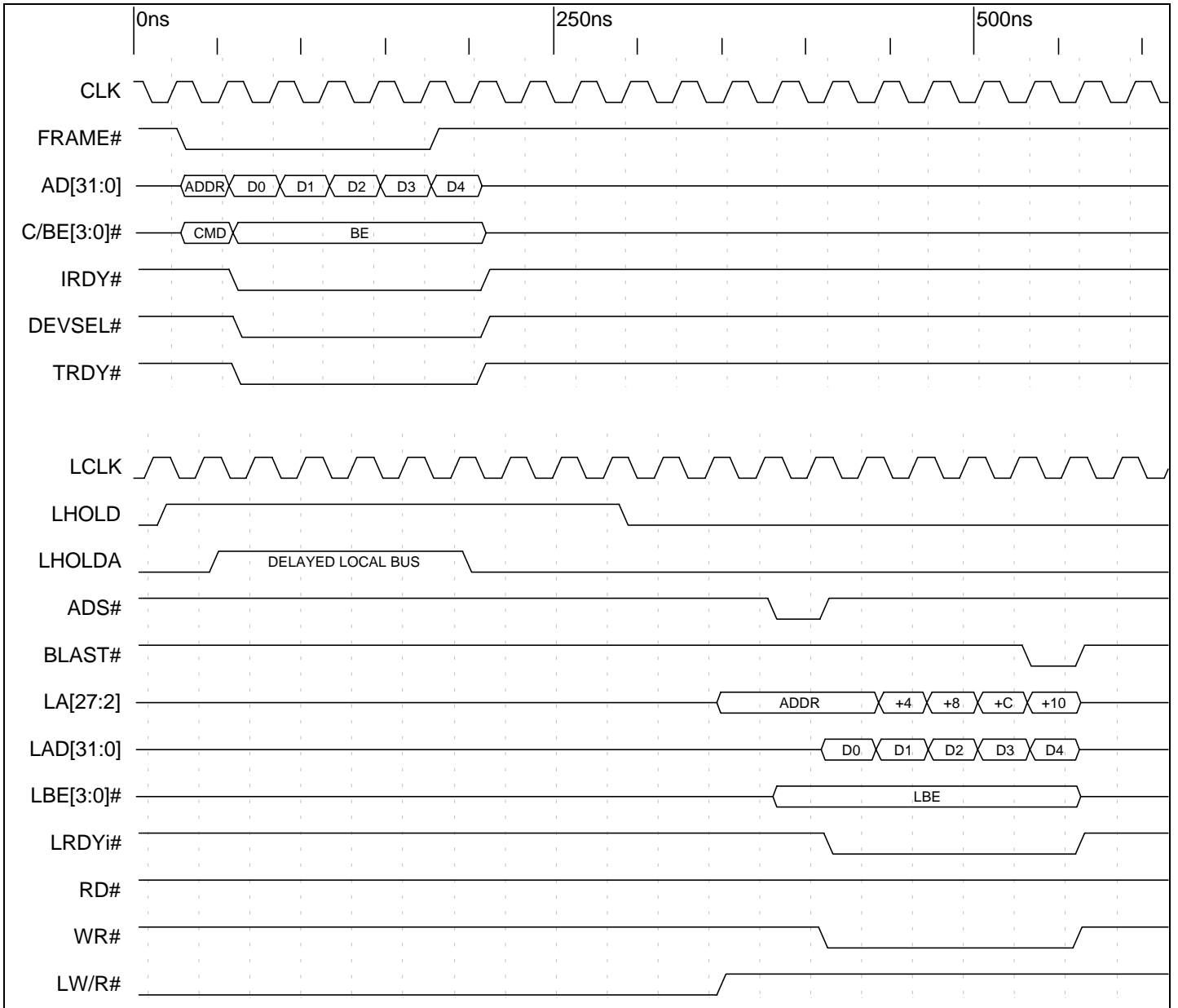
Timing Diagram 9-17. Direct Slave Burst Write with Delayed Local Bus (32 Bit Local Bus)
