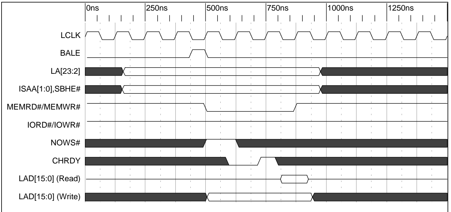
Timing Diagram 9-44. 16 Bit Memory Read/Write Extended ISA Cycle (4 LCLK Shown)
