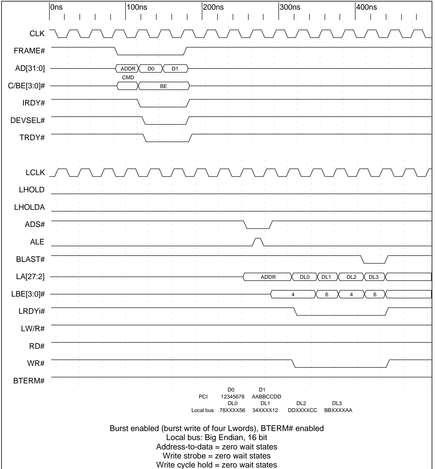
Timing Diagram 9-34. Direct Slave Burst Write and Multiplexed Local Bus (16 Bit Local Bus, J Mode)
