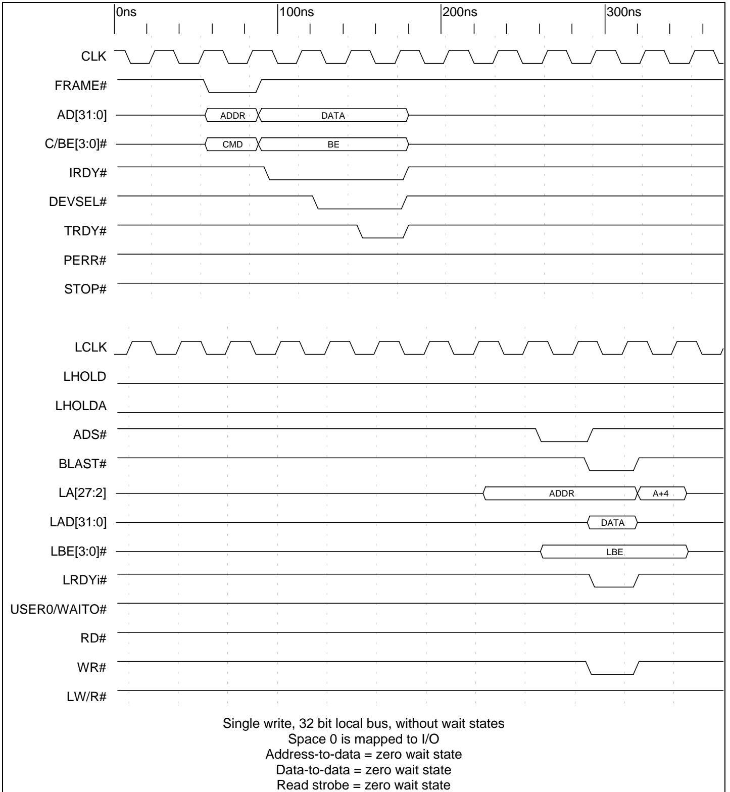
Timing Diagram 9-8. Direct Slave Single Write (32 Bit Local Bus)
