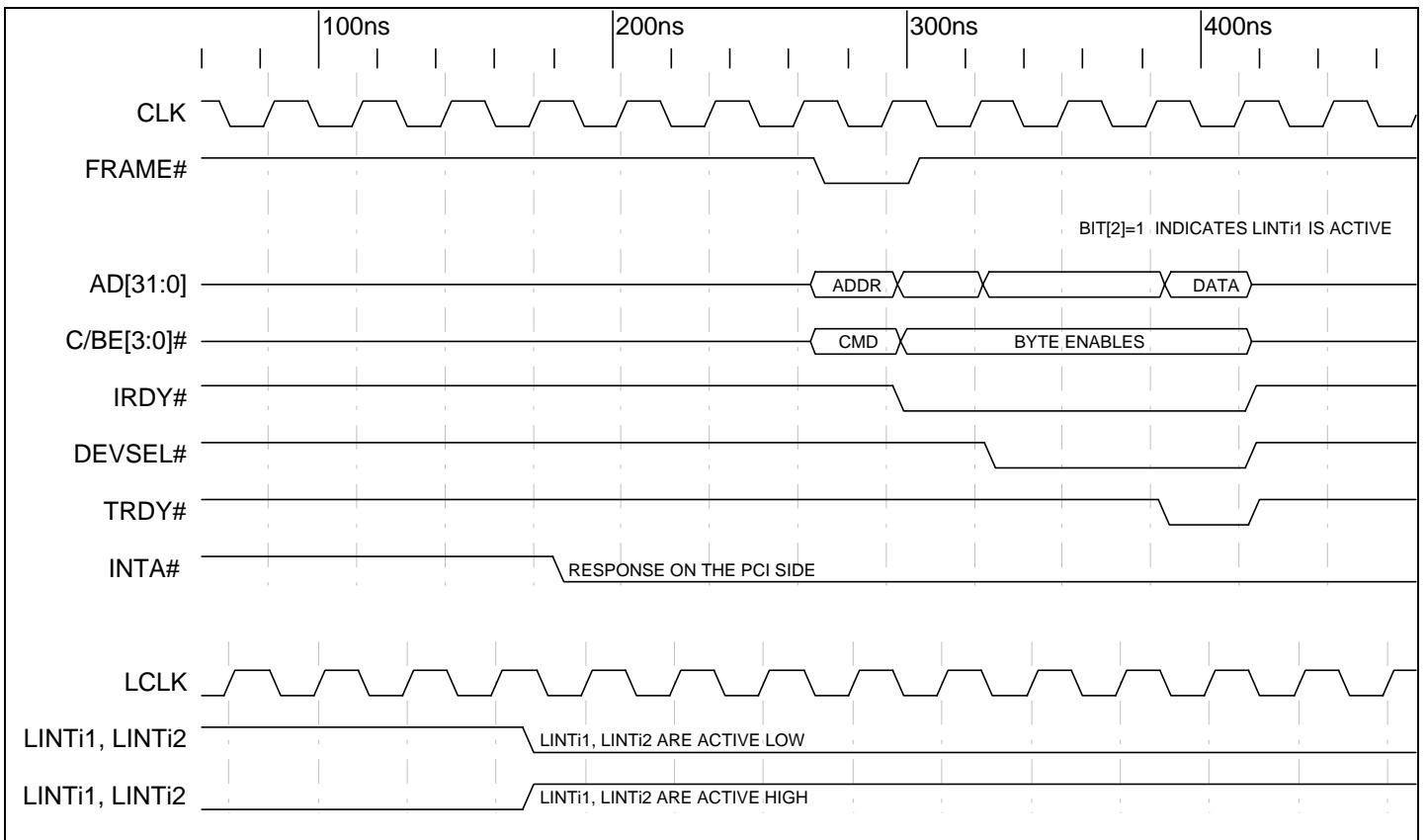
Timing Diagram 9-3. Local LINTi1# Input Asserting PCI Output INTA#
