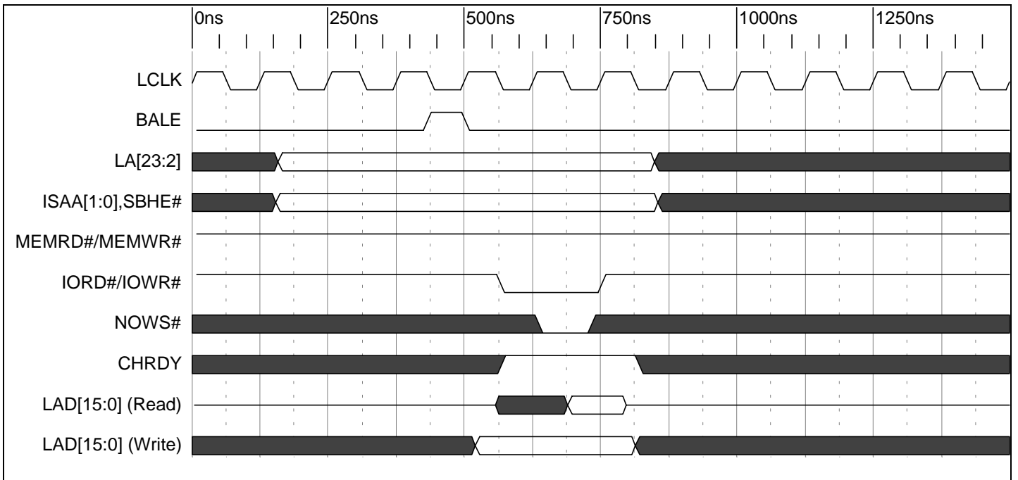
Timing Diagram 9-42. 8 Bit I/O Read/Write Compressed ISA Cycle (3 LCLK Shown)
