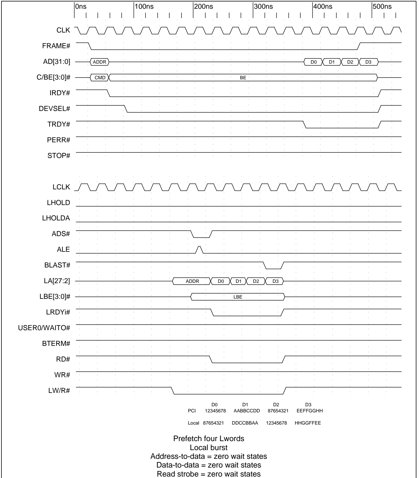
Timing Diagram 9-35. Direct Slave Burst Read and Multiplexed Local Bus (32 Bit Local Bus, J Mode)
