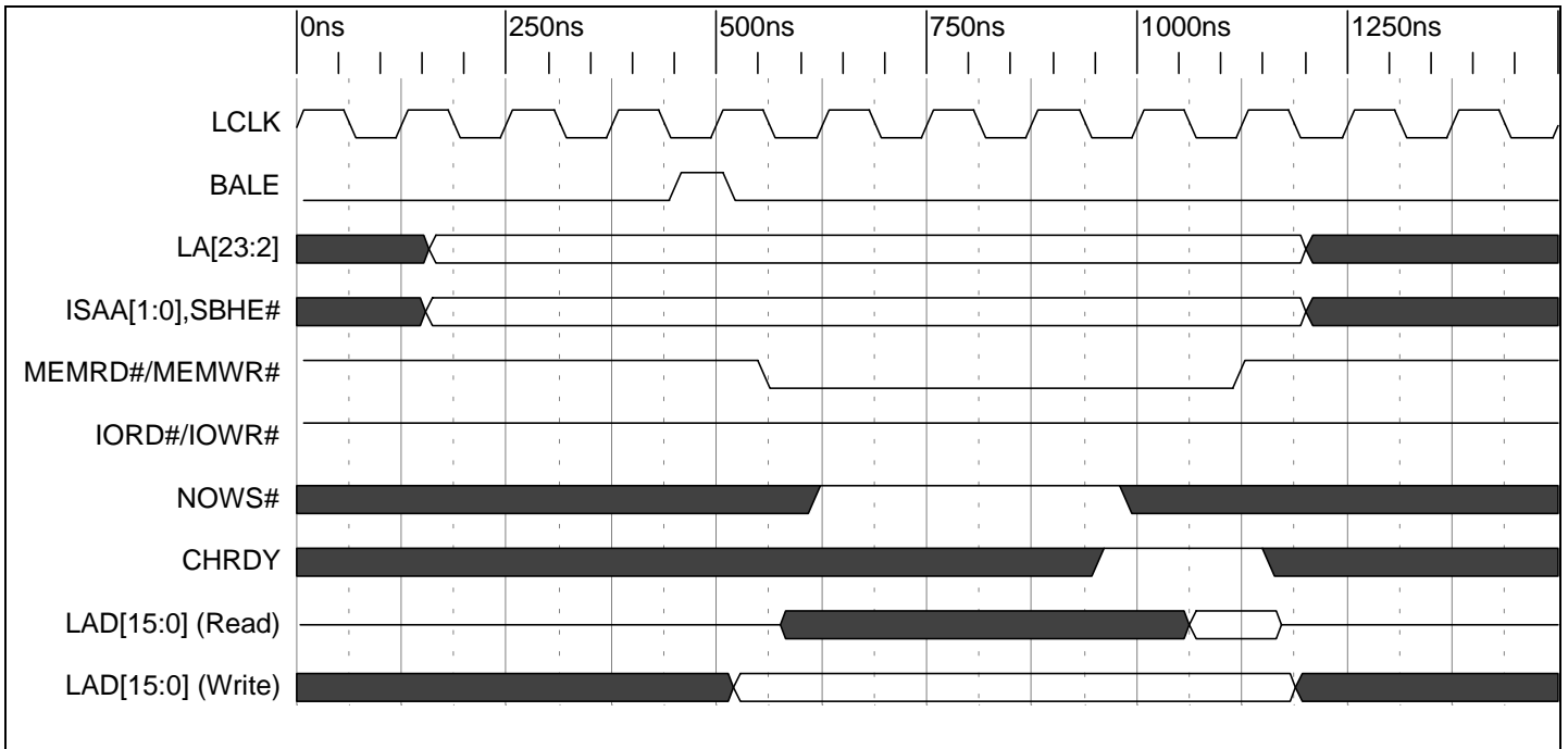
Timing Diagram 9-37. 8 Bit Memory Read/Write Standard ISA Cycle (6 LCLK Shown)
