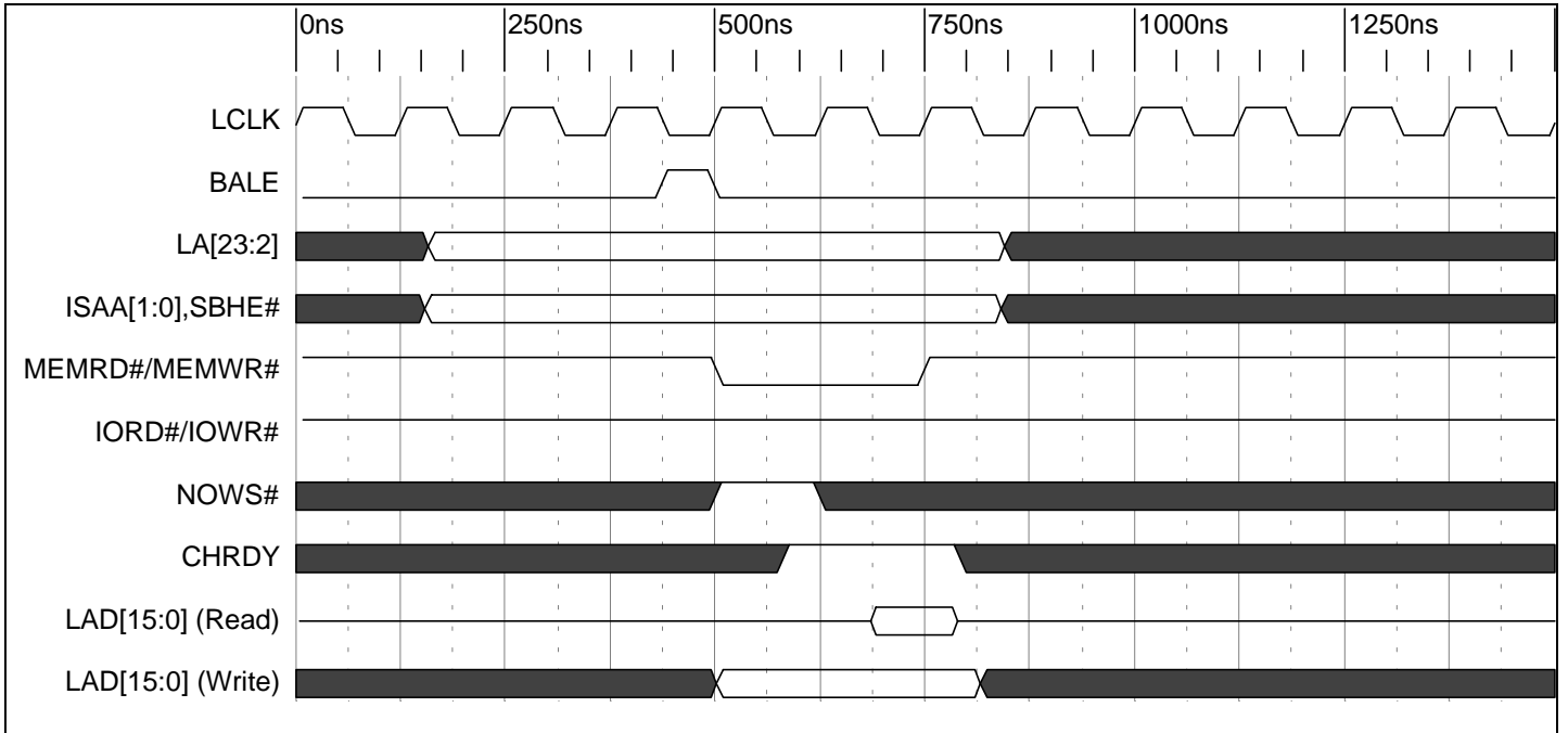
Timing Diagram 9-43. 16 Bit Memory Read/Write Standard ISA Cycle (3 LCLK Shown)
