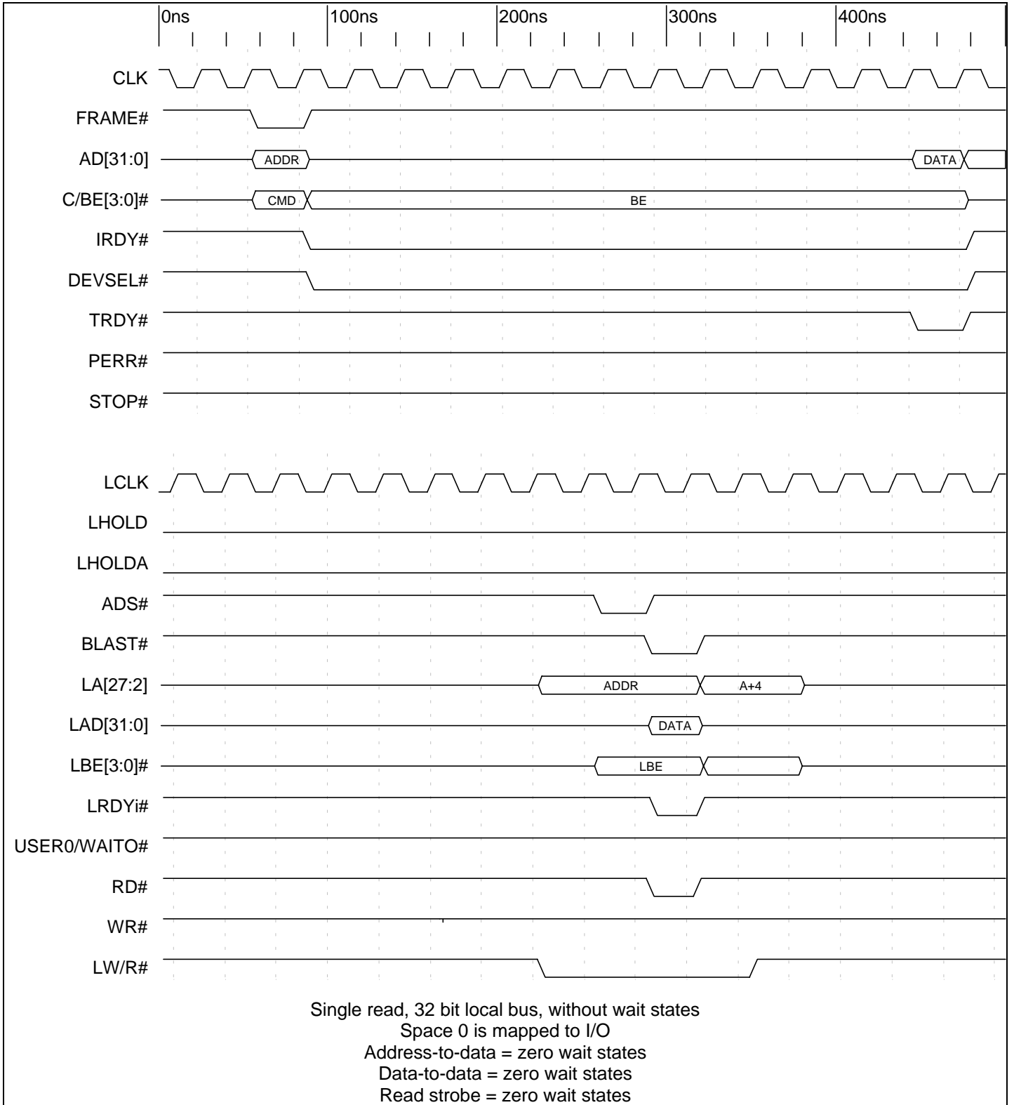
Timing Diagram 9-9. Direct Slave Single Read without Wait States (32 Bit Local Bus)
