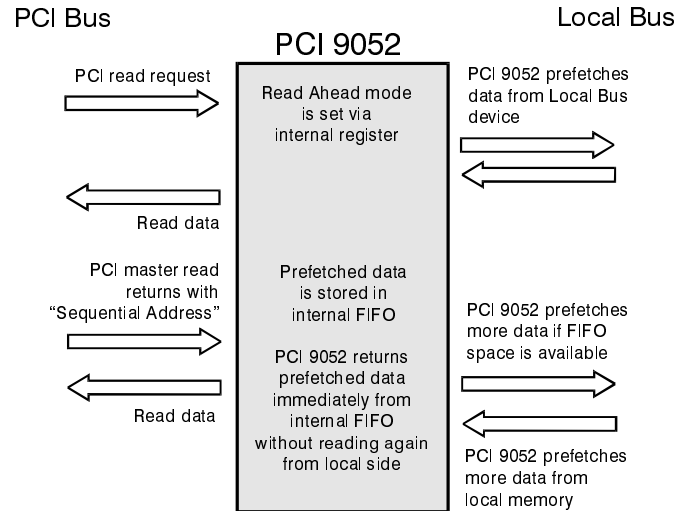
Figure 3-2. PCI 9052 Read Ahead Mode
