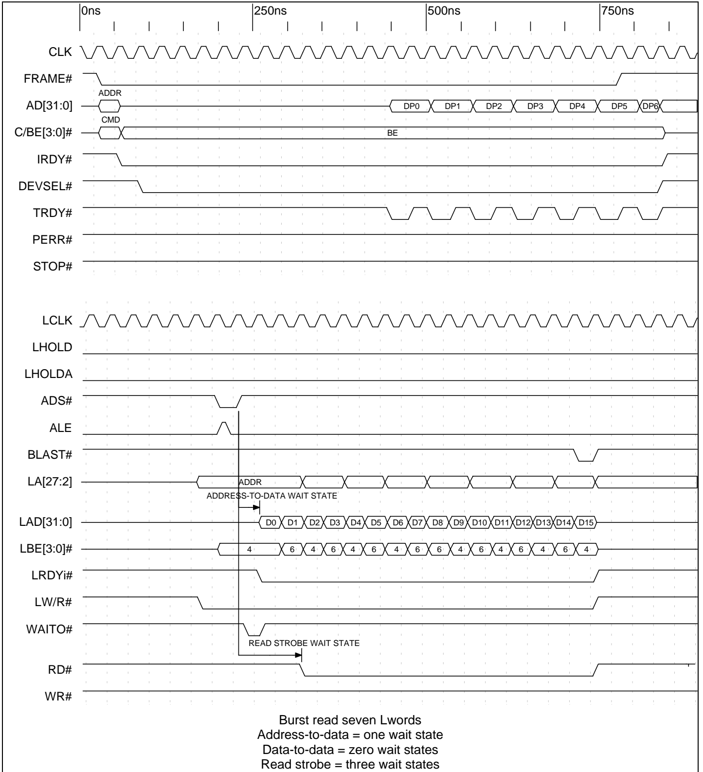
Timing Diagram 9-24. Direct Slave Burst Read with Prefetch of Eight Lwords (16 Bit Local Bus)
