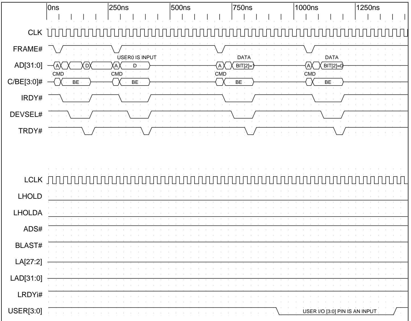
Timing Diagram 9-5. USER I/O Pin 0 Is an Input
