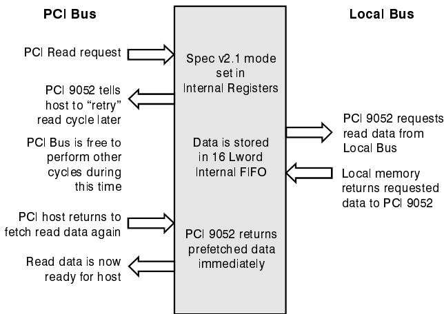
Figure 3-1. PCI Specification v2.1 Delayed Reads
