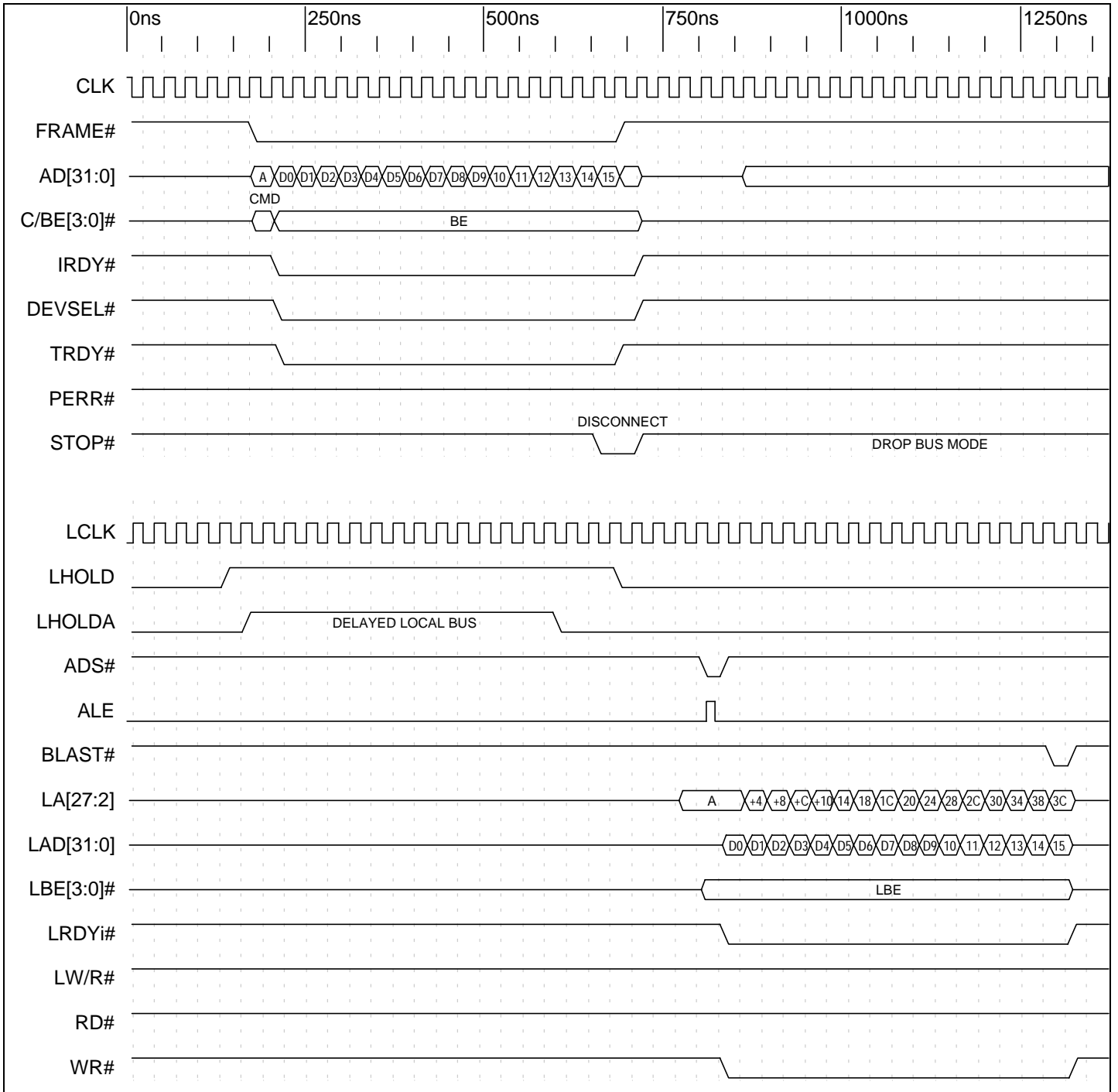
Timing Diagram 9-26. Direct Slave Write PCI Spec v2.1
