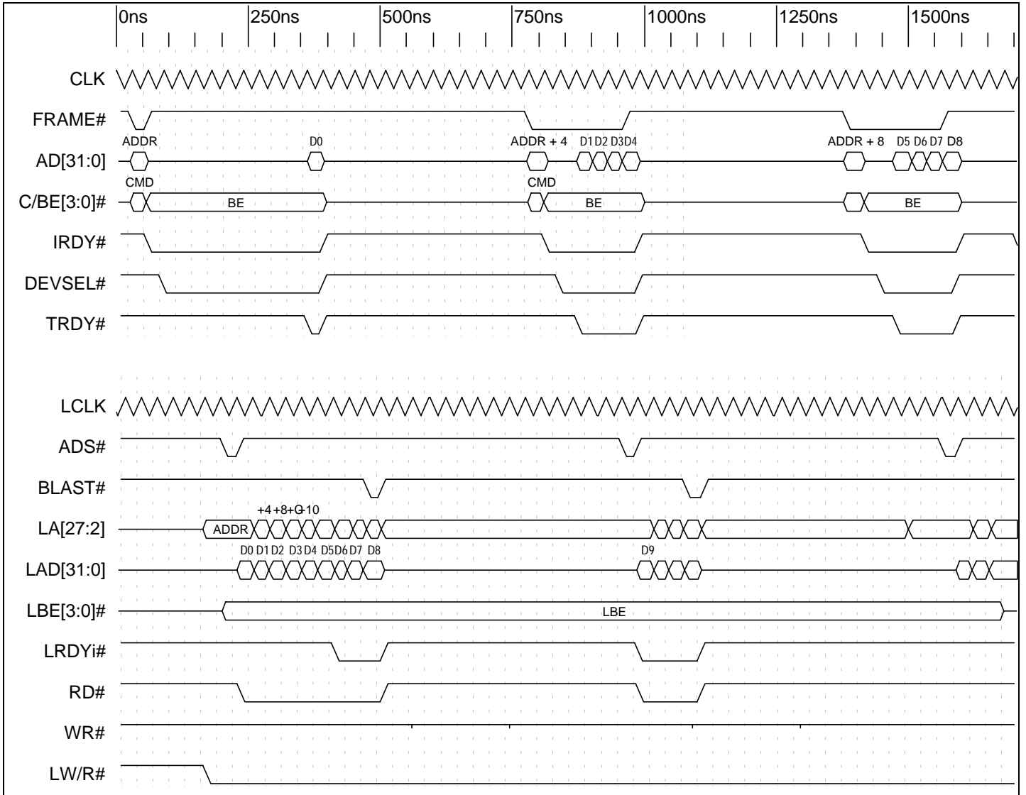
Timing Diagram 9-29. Read Ahead Mode
