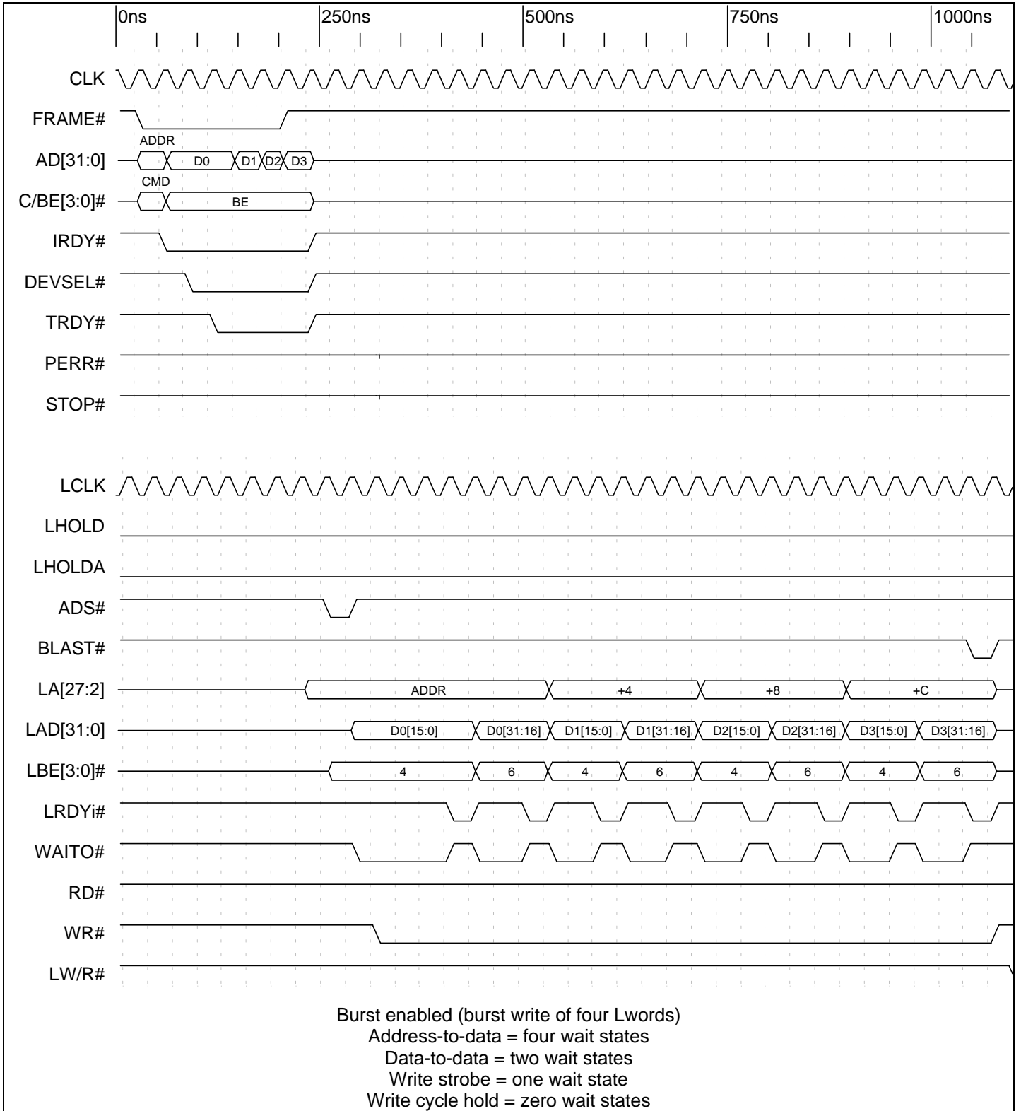
Timing Diagram 9-21. Direct Slave Burst Write (16 Bit Local Bus)
