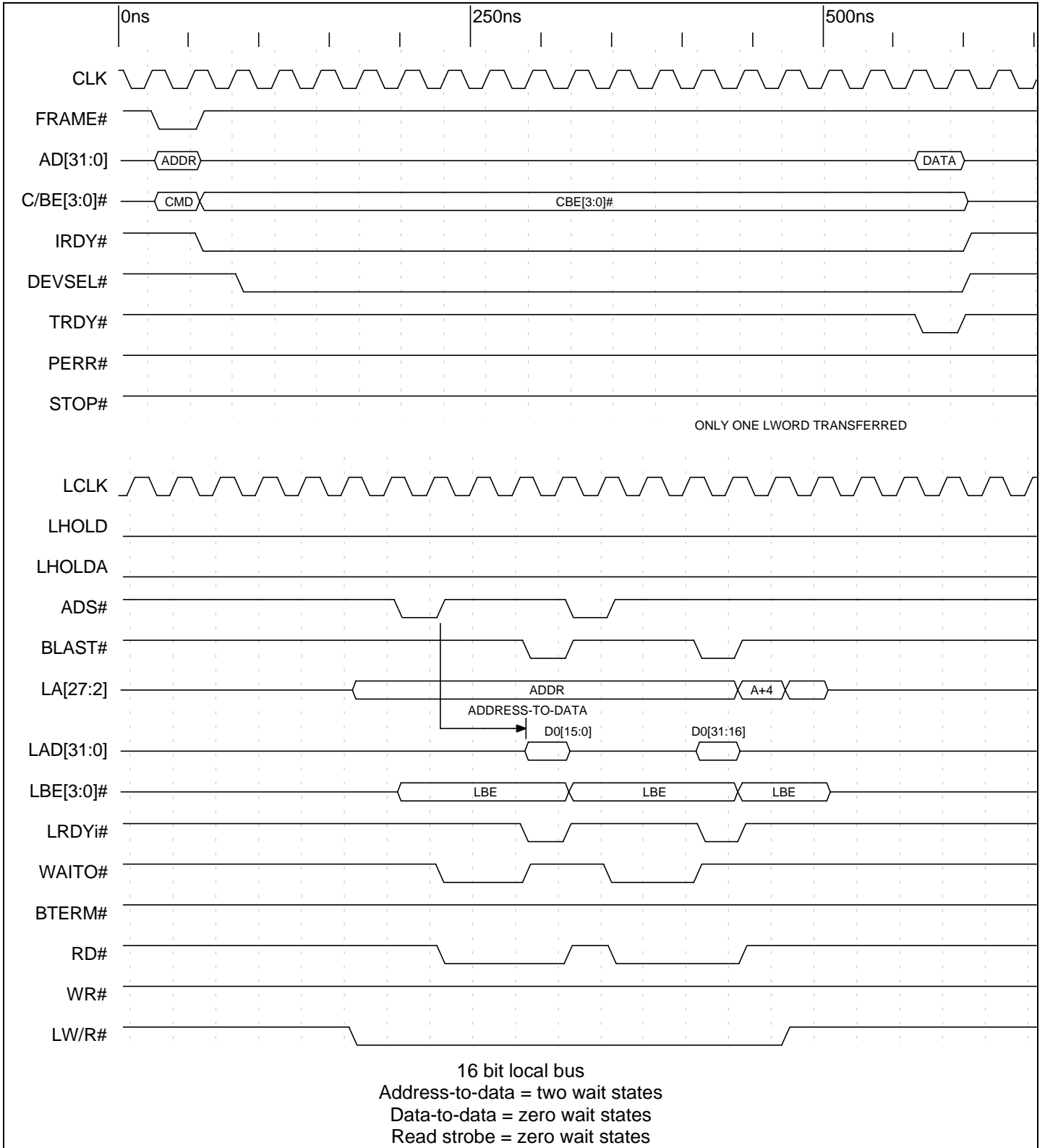
Timing Diagram 9-14. Direct Slave Non-Burst Read with Unaligned PCI Address (32 Bit Local Bus)
