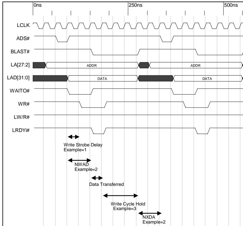
Figure 2-1. PCI 9052 Single Cycle Write
