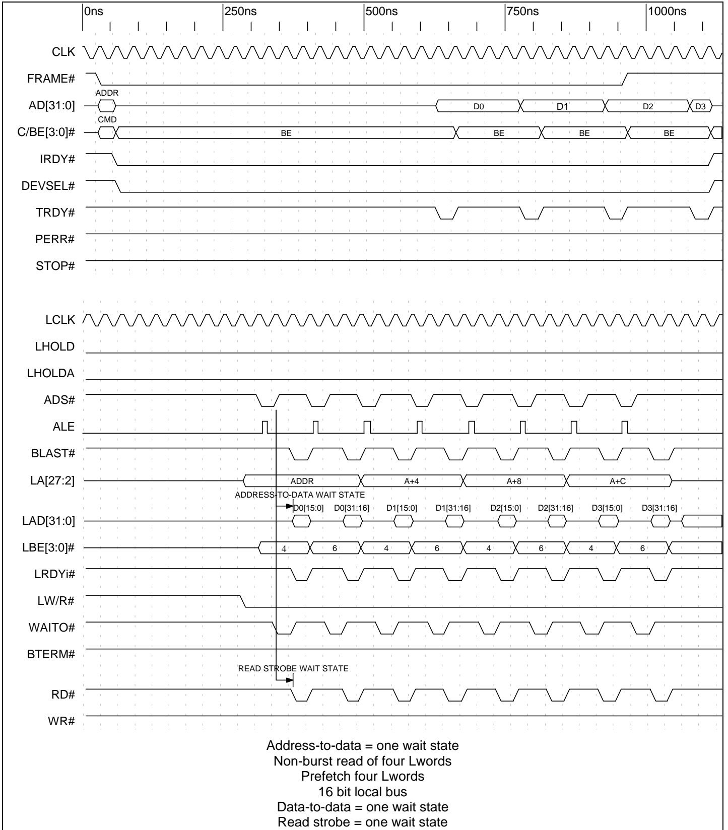
Timing Diagram 9-15. Direct Slave Non-Burst Read with Prefetch (16 Bit Local Bus)
