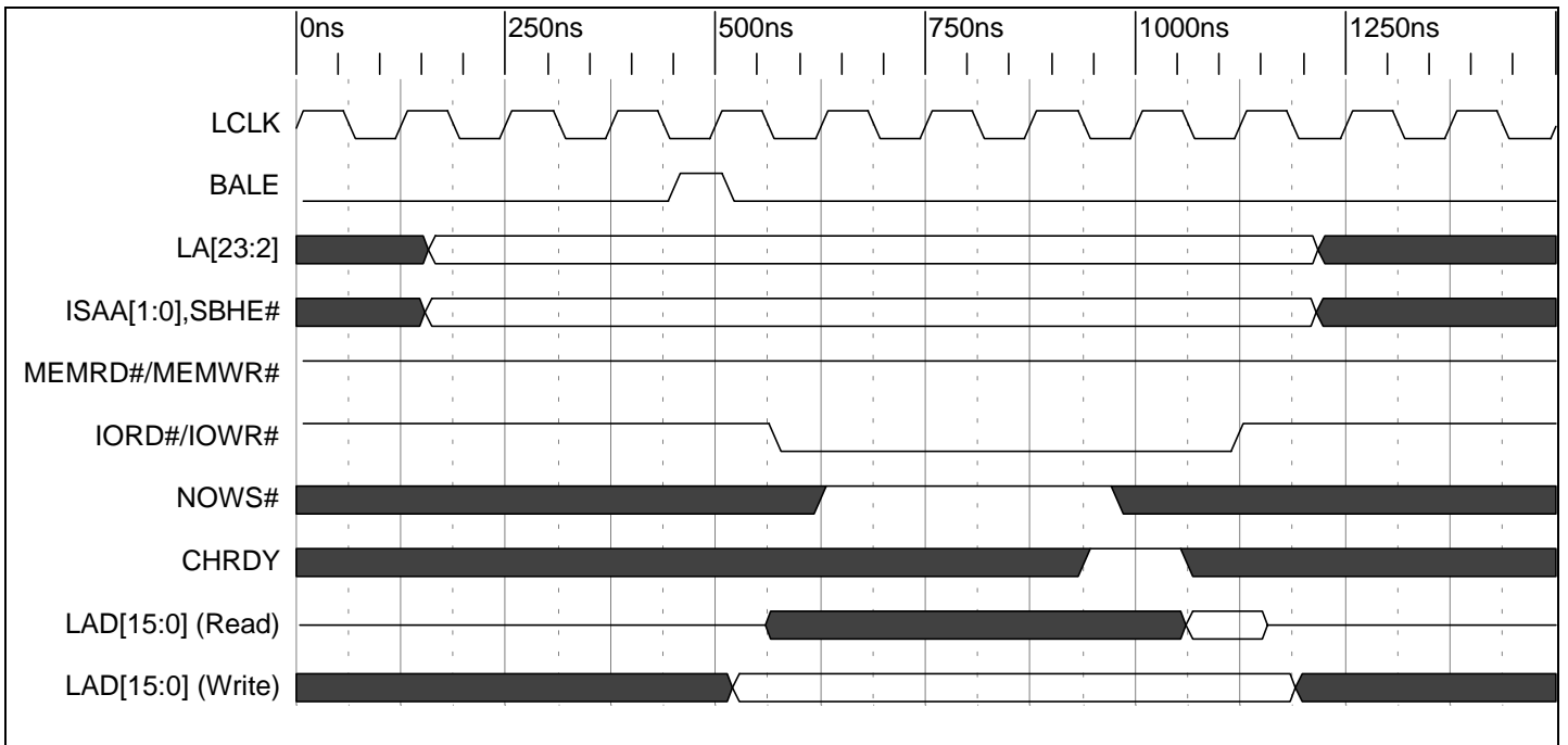
Timing Diagram 9-40. 8 Bit I/O Read/Write Standard ISA Cycle (6 LCLK Shown)
