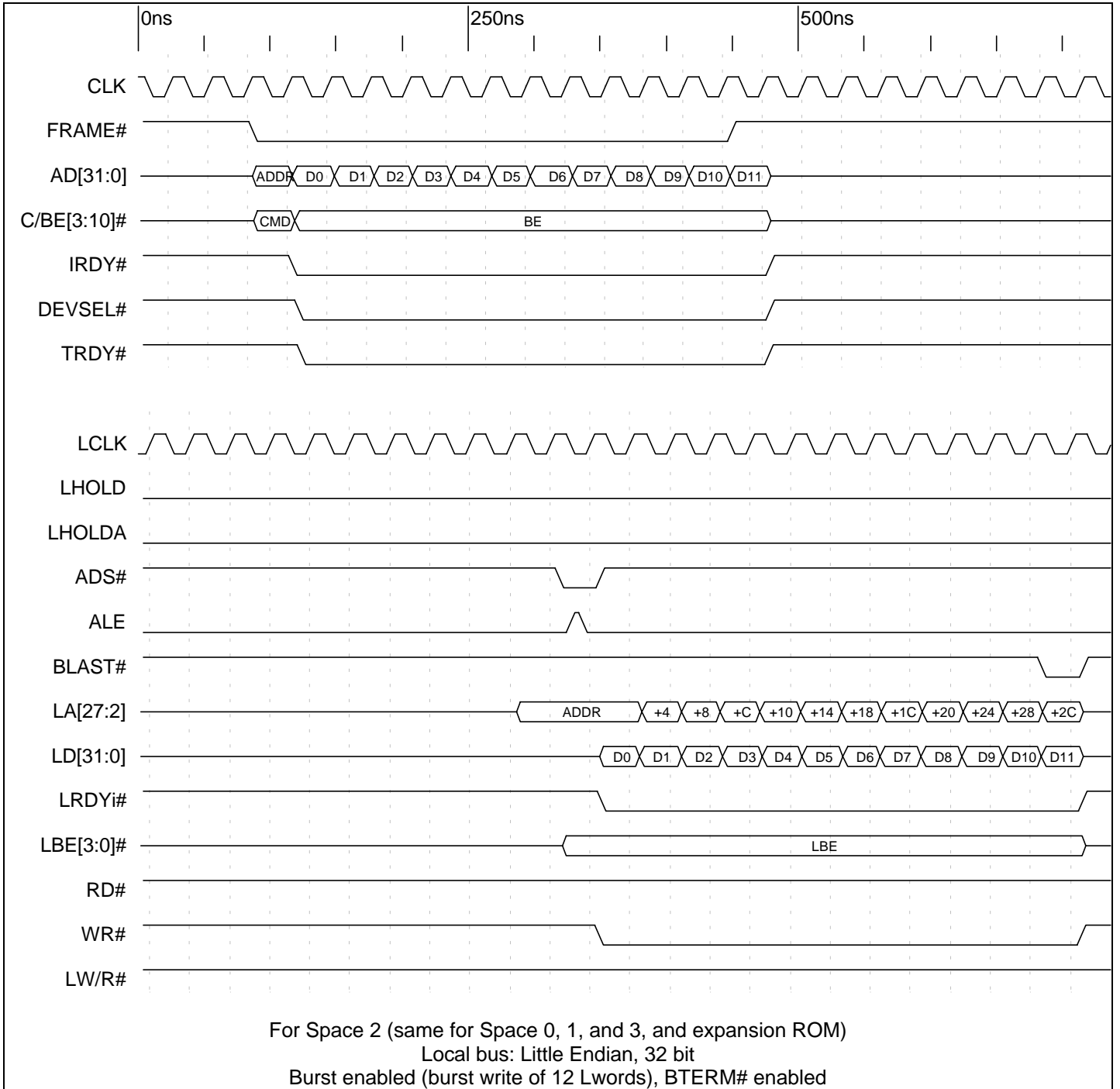
Timing Diagram 9-18. Direct Slave Burst Write with BTERM# Enabled (32 Bit Local Bus)
