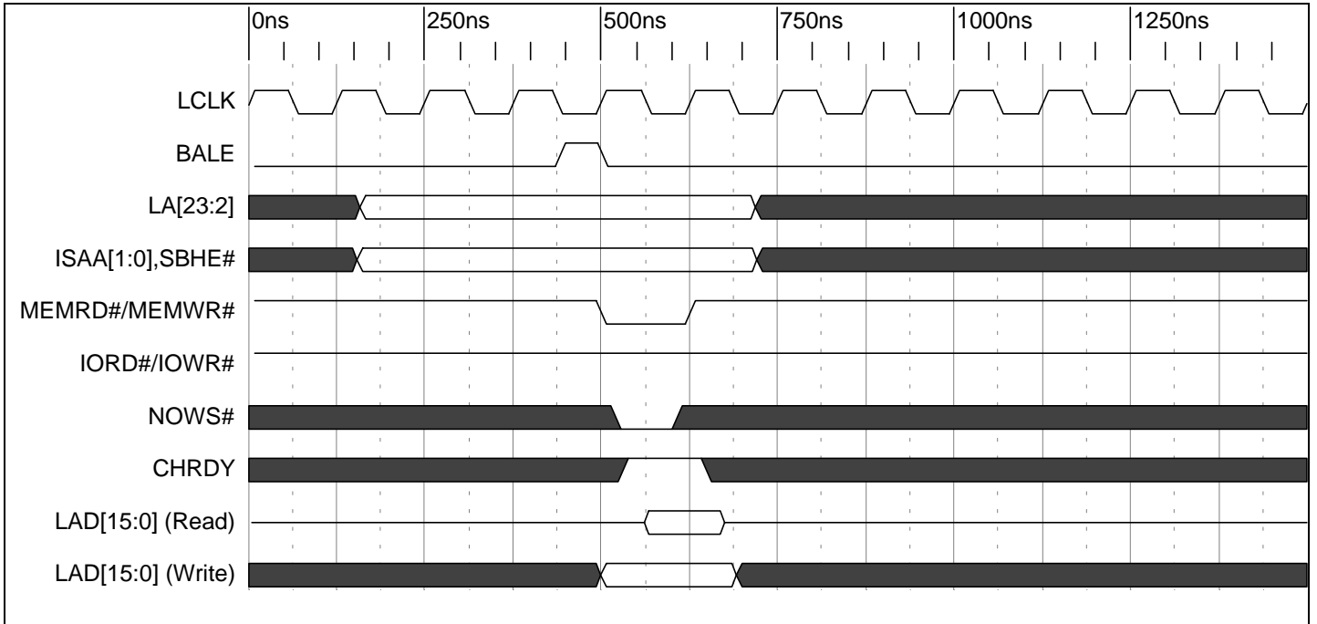
Timing Diagram 9-45. 16 Bit Memory Read/Write Compressed ISA Cycle (2 LCLK Shown)
