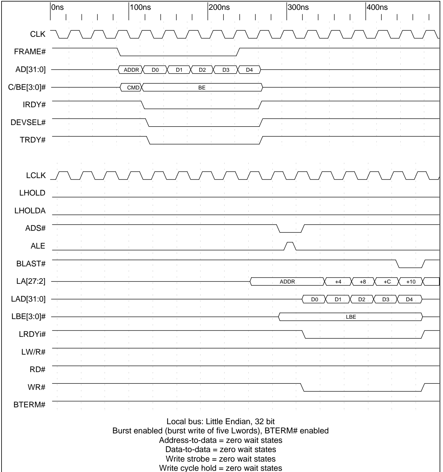
Timing Diagram 9-20. Direct Slave Burst Write with BTERM# Enabled (32 Bit Local Bus)
