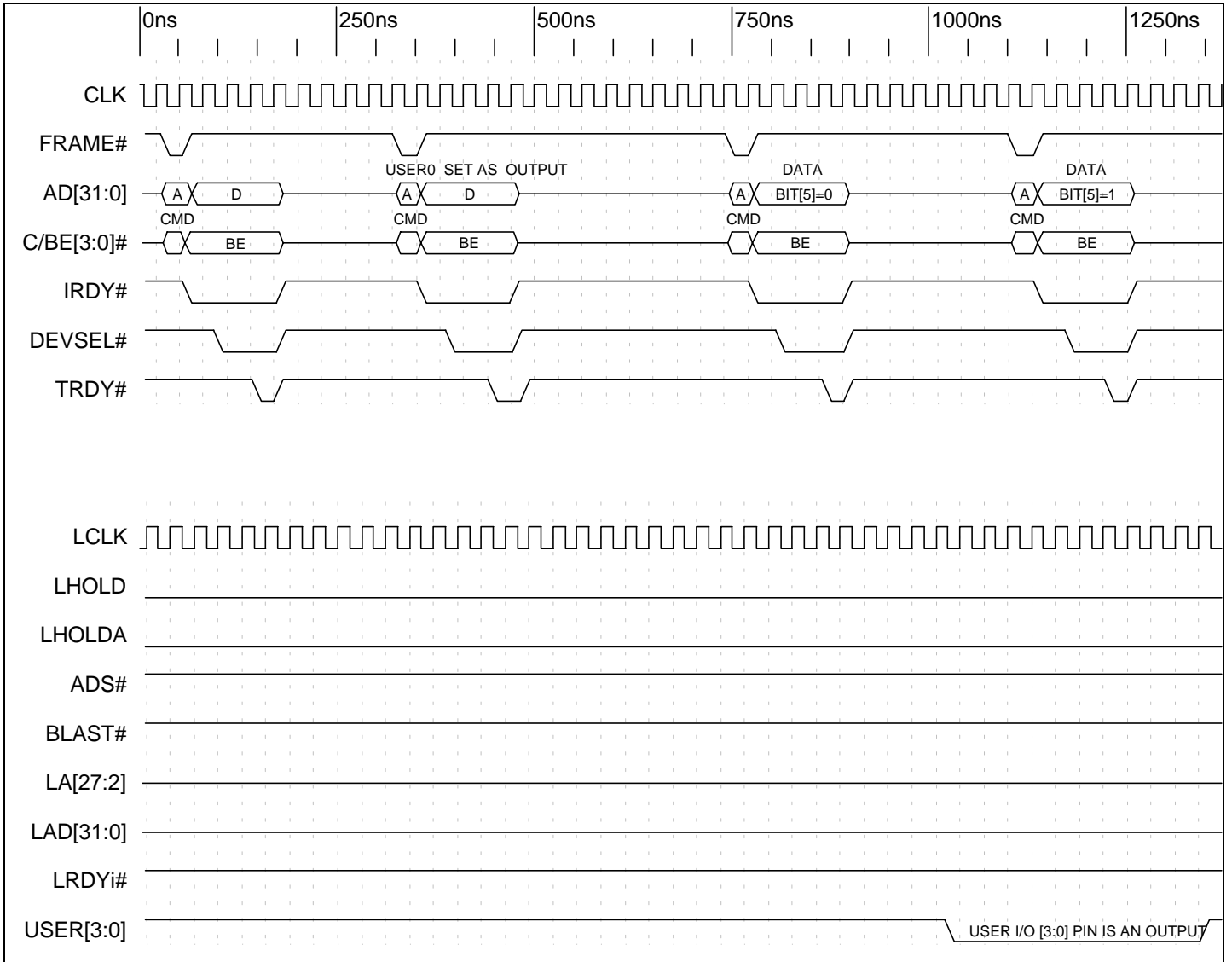
Timing Diagram 9-6. USER I/O Pin 0 Is an Output
