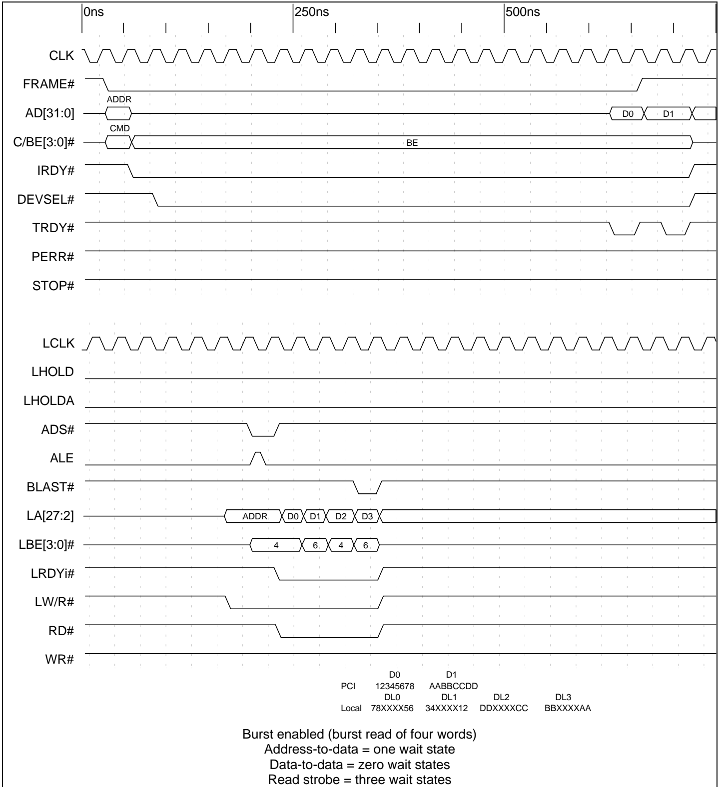
Timing Diagram 9-36. Direct Slave Burst Read and Multiplexed Local Bus (16 Bit Local Bus, J Mode)
