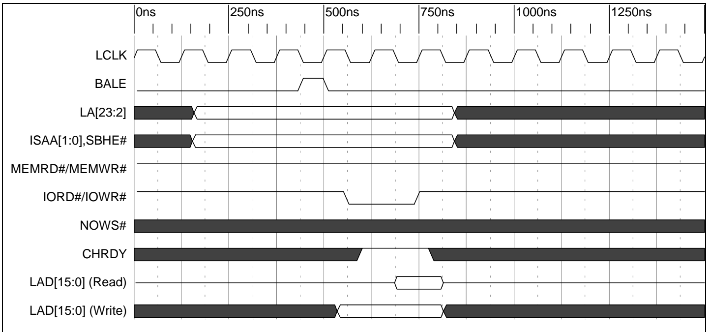
Timing Diagram 9-46. 16 Bit I/O Read/Write Standard ISA Cycle (3 LCLK Shown)
