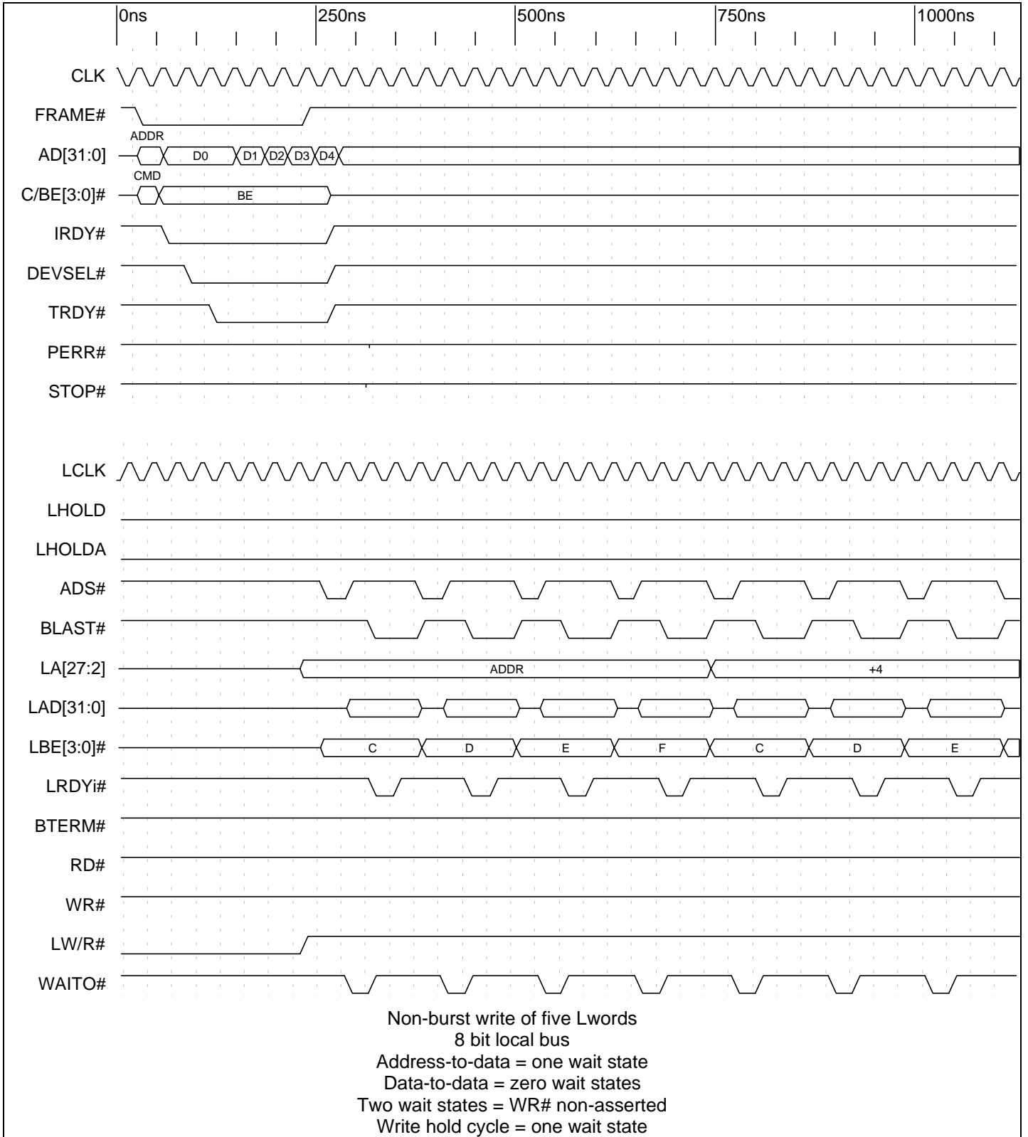
Timing Diagram 9-12. Direct Slave Non-Burst Write (8 Bit Local Bus)
