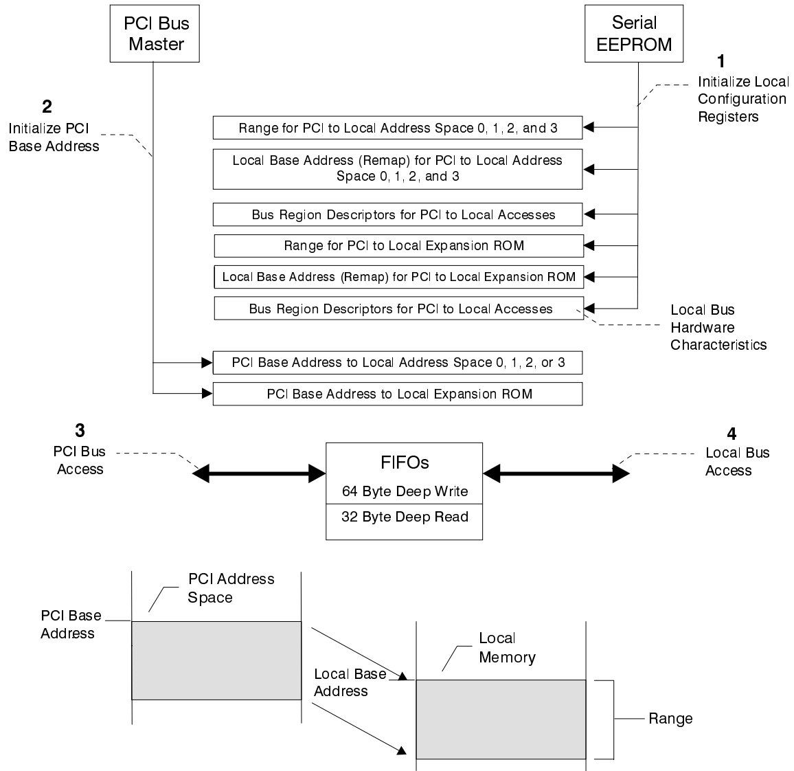
Figure 3-5. PCI Master Direct Access of Local Bus
