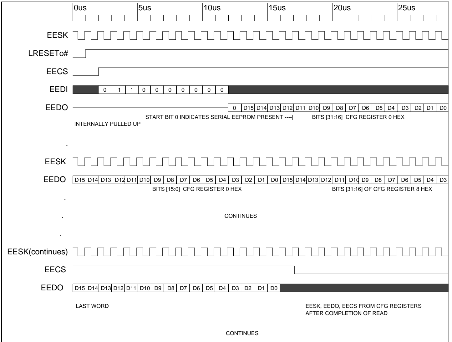
Timing Diagram 9-1. Initialization from Serial EEPROM
