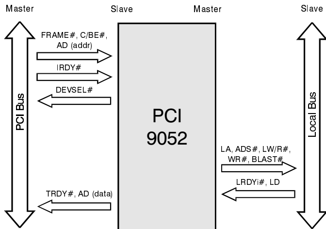
Figure 3-4. Direct Slave Read
