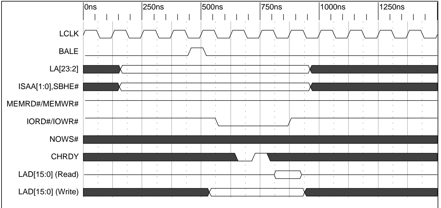
Timing Diagram 9-47. 16 Bit I/O Read/Write Extended ISA Cycle (4 LCLK Shown)
