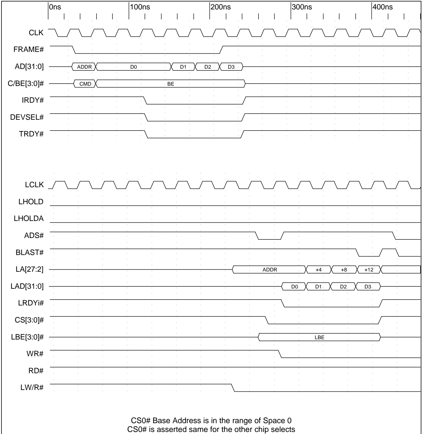
Timing Diagram 9-7. Chip Select 0
