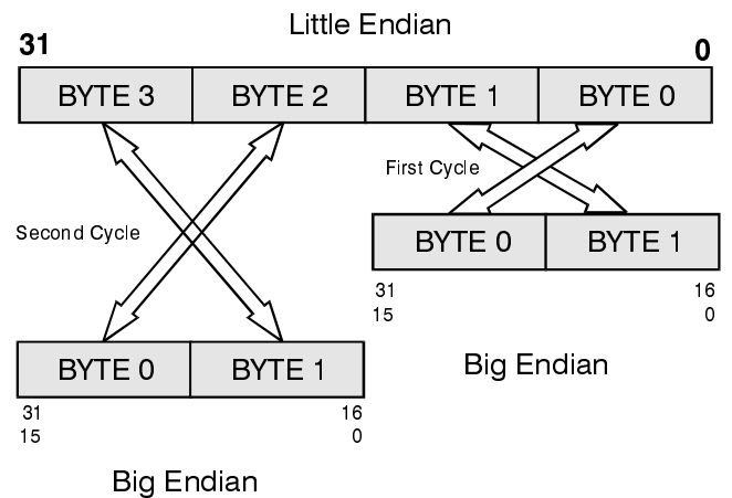
Figure 2-4. Big/Little Endian—16 Bit Local Bus
