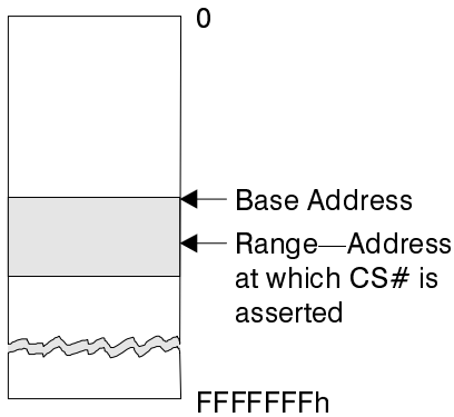
Figure 2-6. Chip Select Base Address and Range
