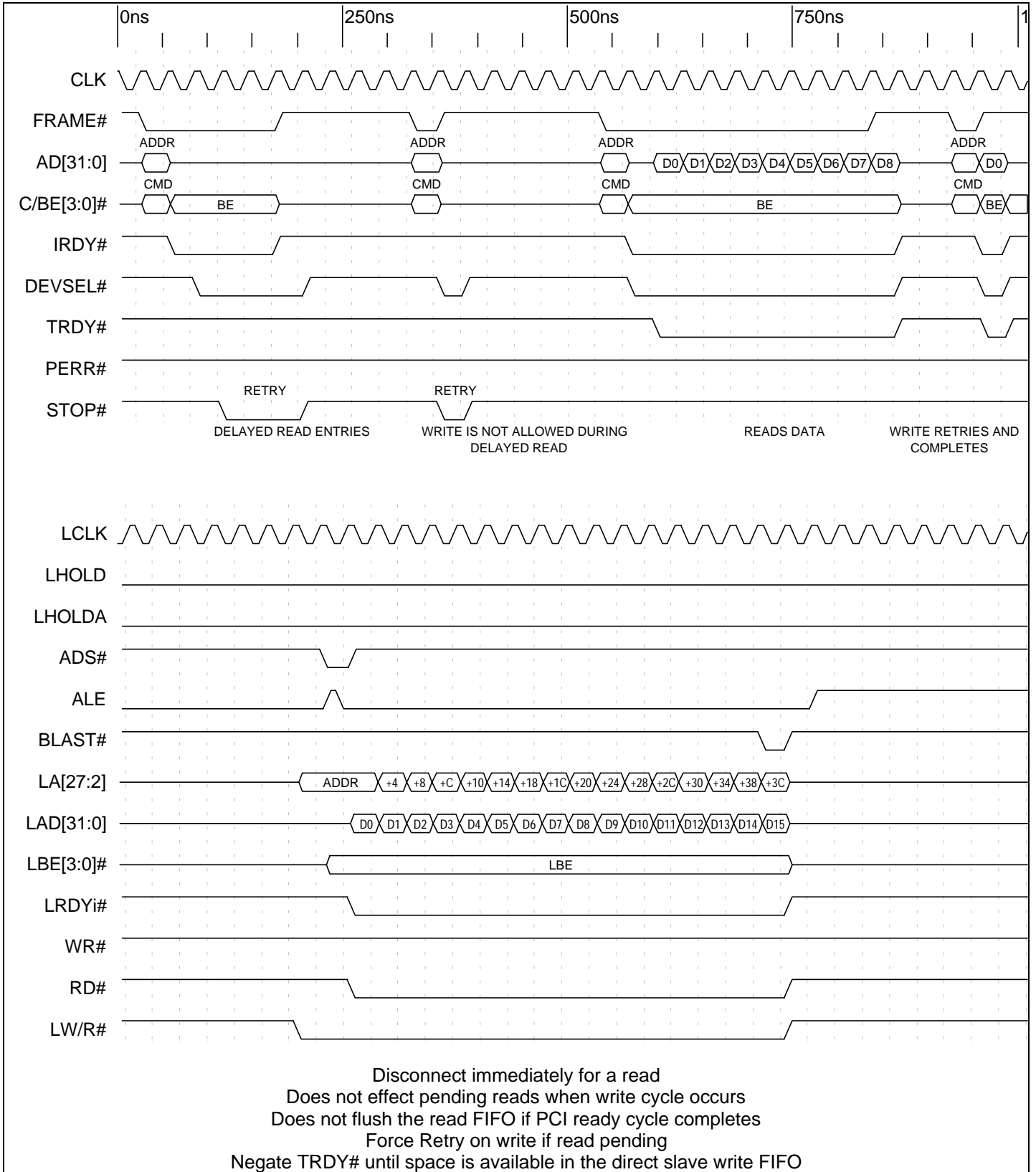
Timing Diagram 9-27. Direct Slave Read PCI Spec v2.1
