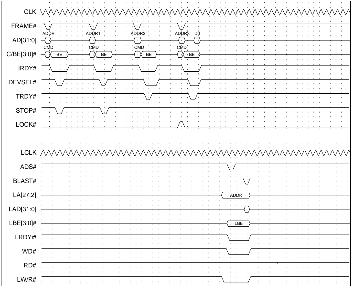
Timing Diagram 9-30. PCI Lock Mode
