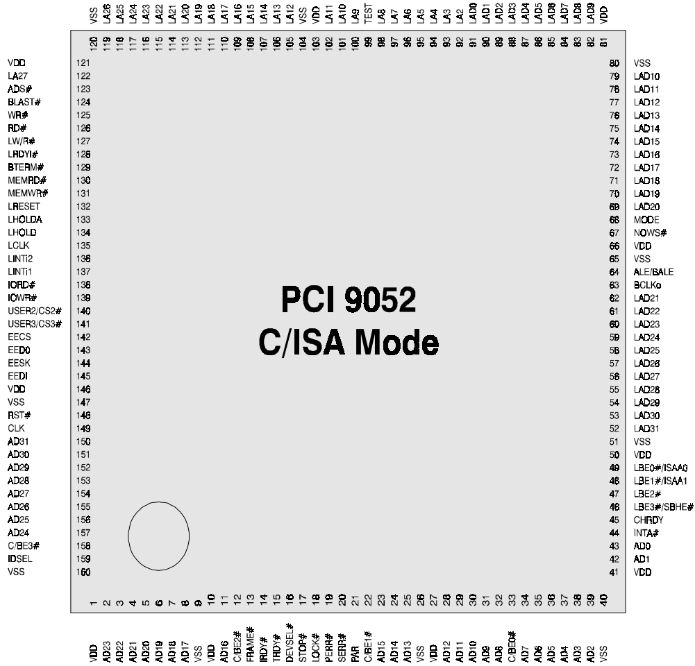
Figure 8-4. PCI 9052 Pin Out (C/ISA Mode)
