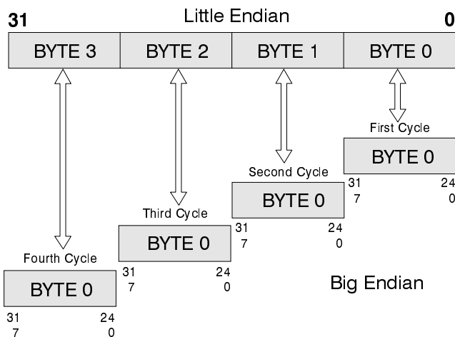
Figure 2-5. Big/Little Endian—8 Bit Local Bus
