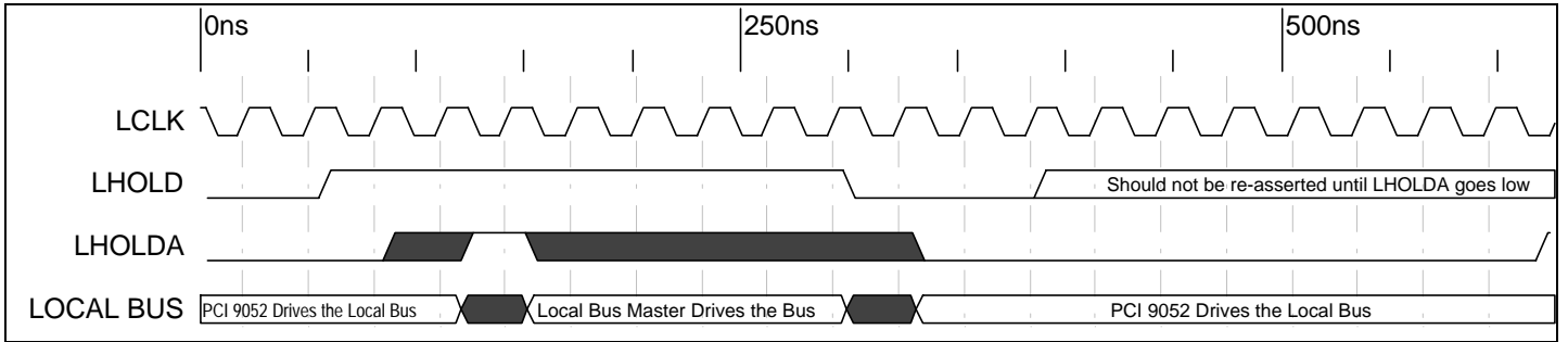
Timing Diagram 9-2. Local Bus Arbitration
