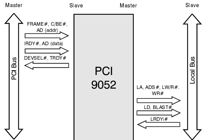
Figure 3-3. Direct Slave Write
