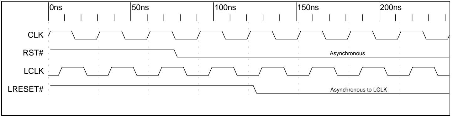
Timing Diagram 9-4. PCI RST# Asserting Local Output LRESET#
