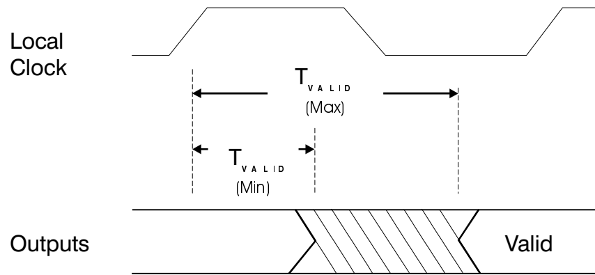
Figure 7-2. PCI 9052 Local Input Setup and Hold Waveform
