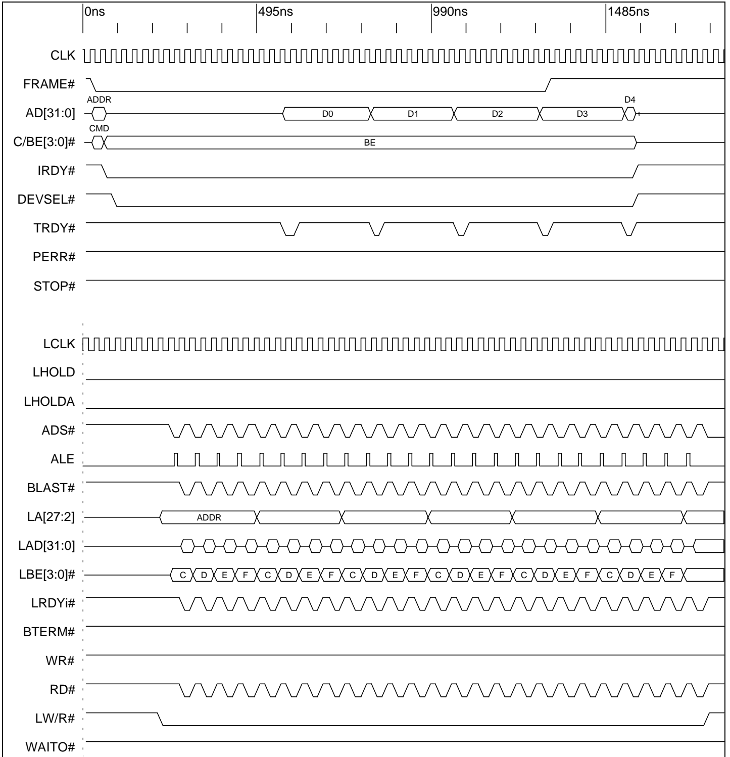
Timing Diagram 9-16. Direct Slave Non-Burst Read with Prefetch (8 Bit Local Bus)
