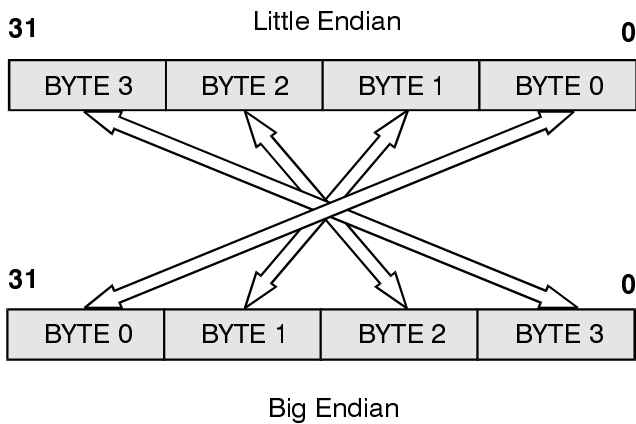
Figure 2-3. Big/Little Endian—32 Bit Local Bus
