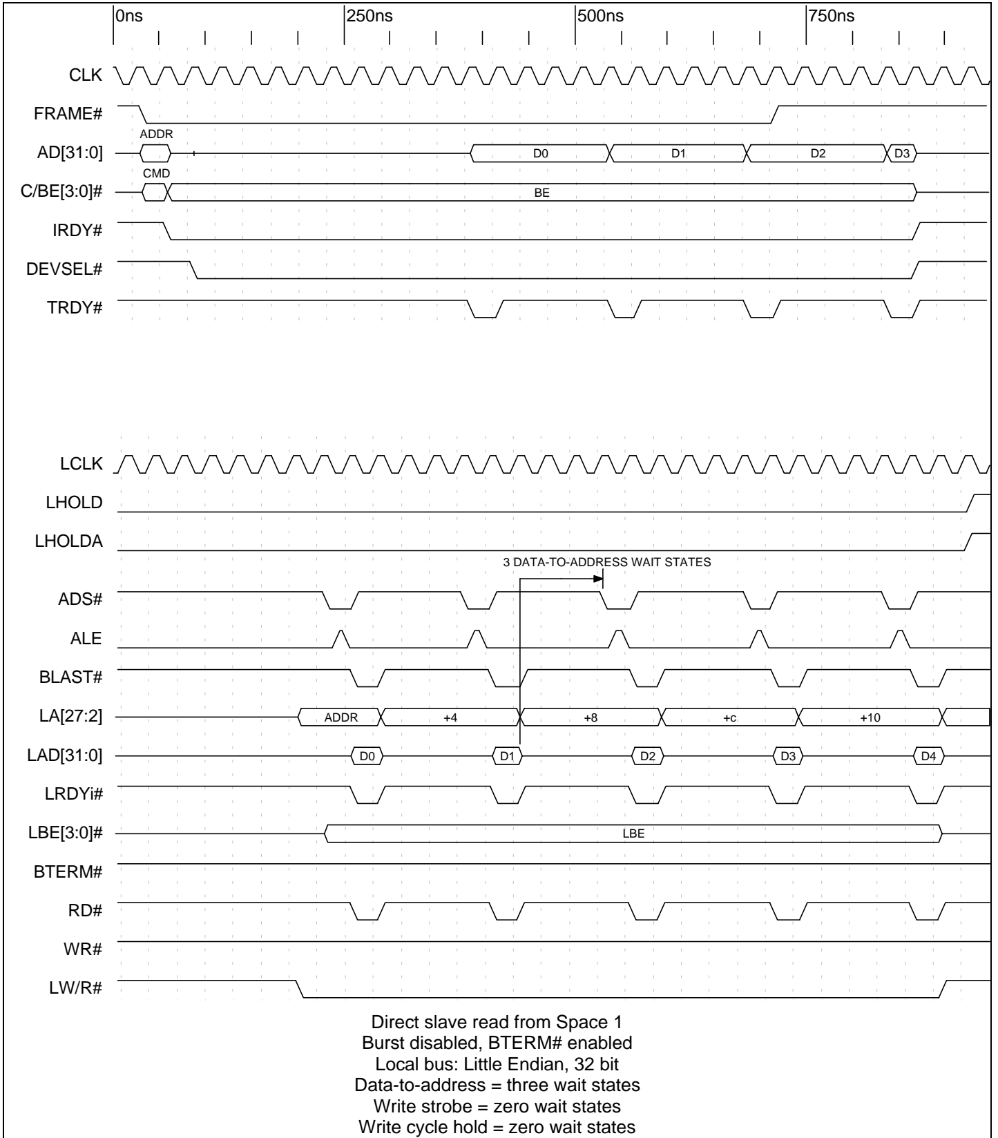
Timing Diagram 9-13. Direct Slave Non-Burst Read with BTERM# Enabled (32 Bit Local Bus)
