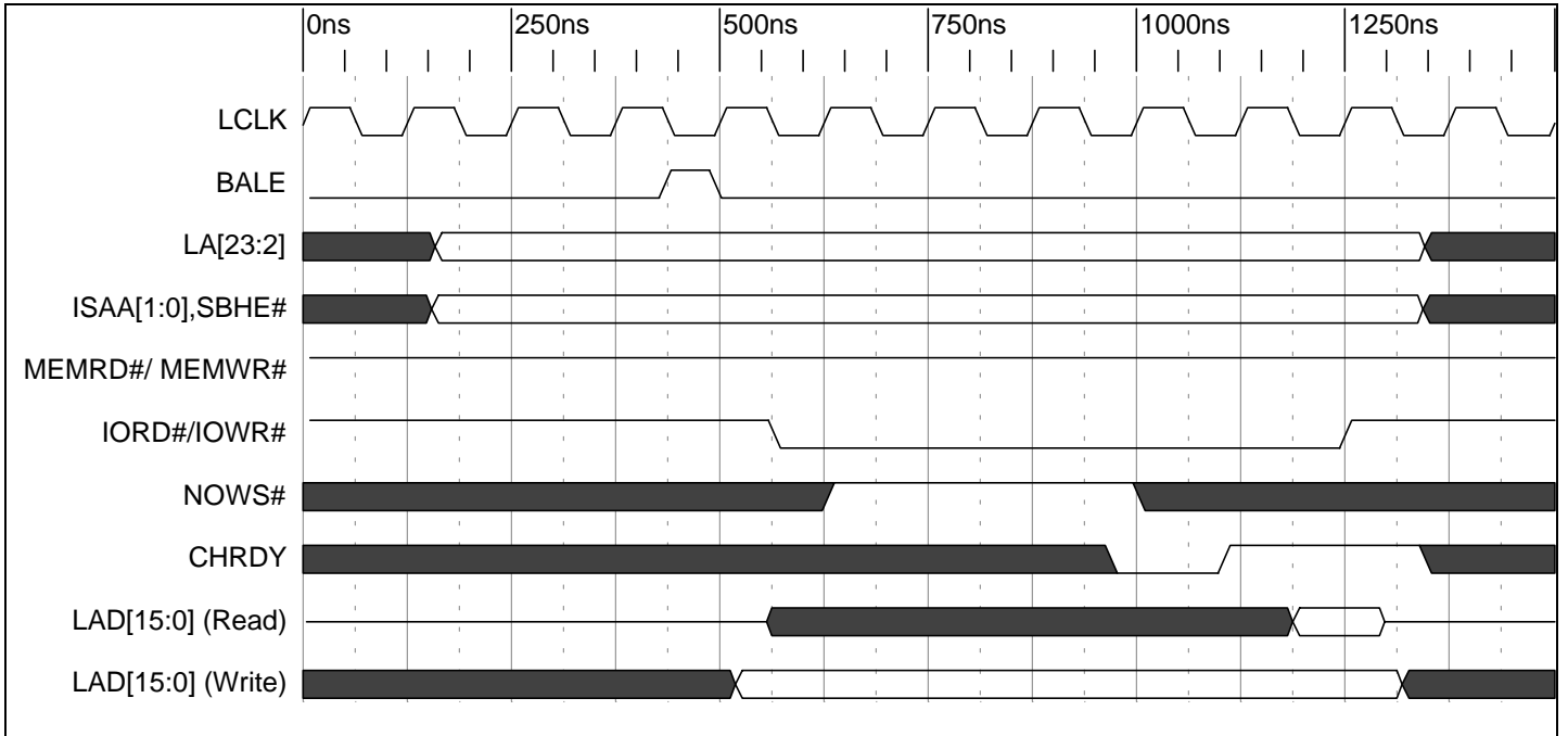
Timing Diagram 9-41. 8 Bit I/O Read/Write Extended ISA Cycle (7 LCLK Shown)
