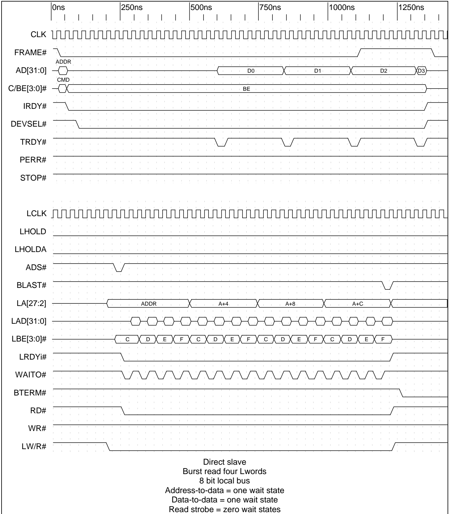
Timing Diagram 9-25. Direct Slave Burst Read with Prefetch of Four Lwords (8 Bit Local Bus)
