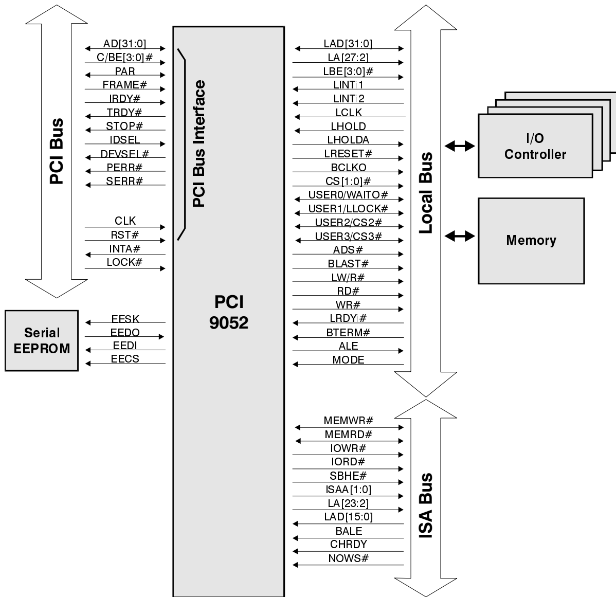
Figure 1-1. PCI 9052 Signal Interfaces
