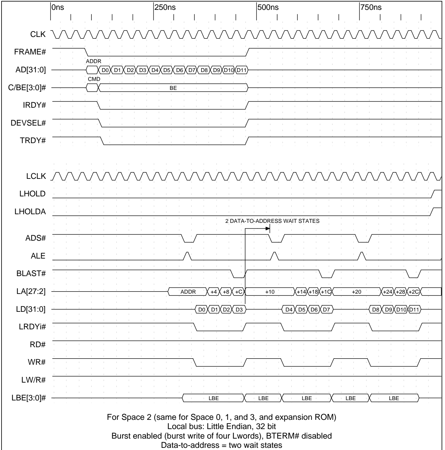
Timing Diagram 9-19. Direct Slave Burst Write with BTERM# Disabled and Wait States (32 Bit Local Bus)
