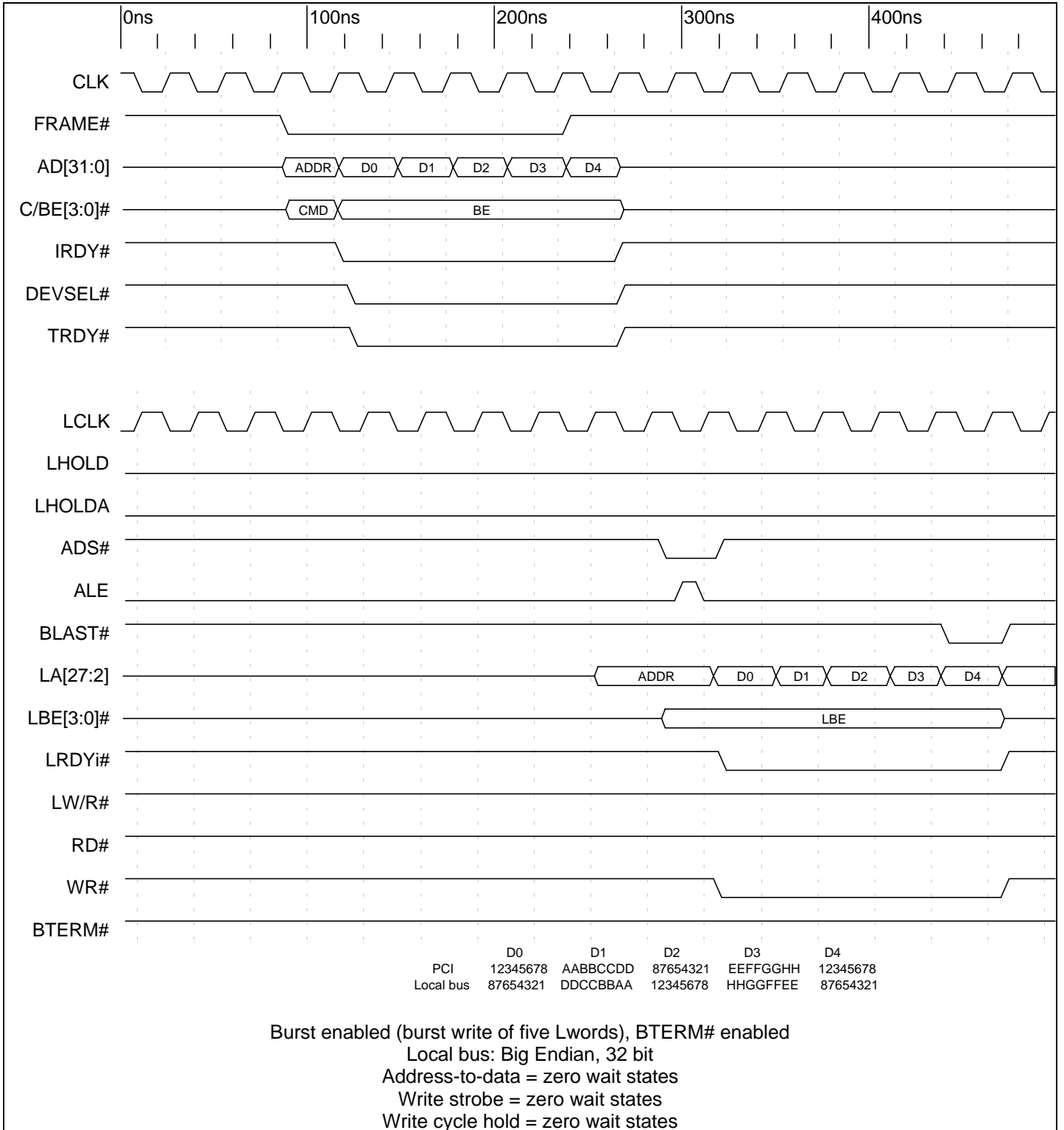
Timing Diagram 9-33. Direct Slave Burst Write and Multiplexed Local Bus (32 Bit Local Bus, J Mode)
