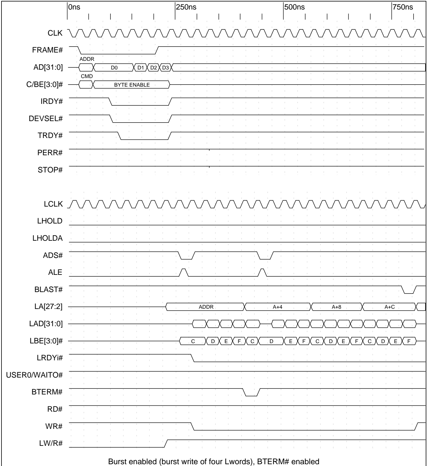
Timing Diagram 9-22. Direct Slave Burst Write with BTERM# Enabled (8 Bit Local Bus)
