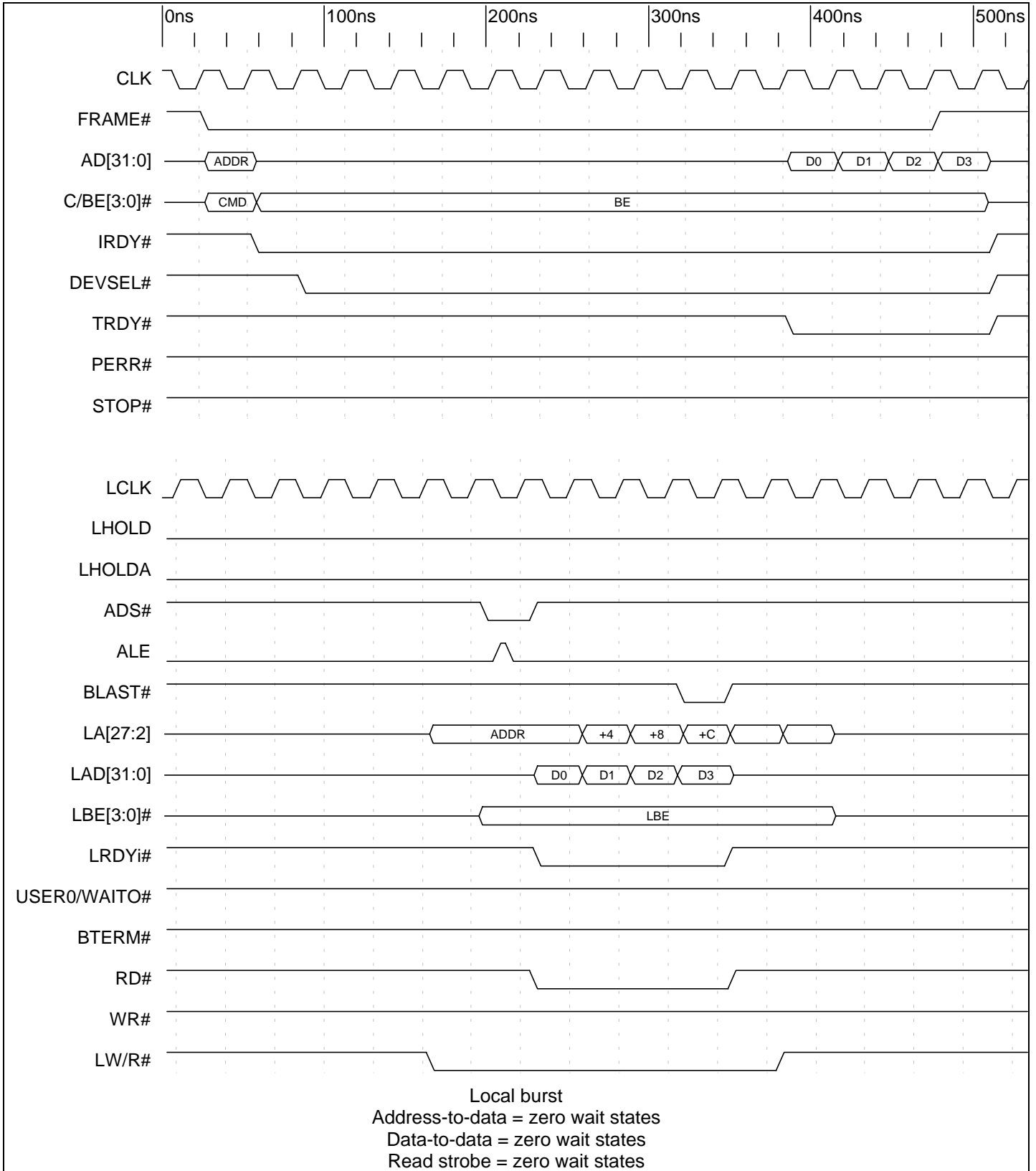
Timing Diagram 9-23. Direct Slave Burst Read with Prefetch of Four Lwords (32 Bit Local Bus)
