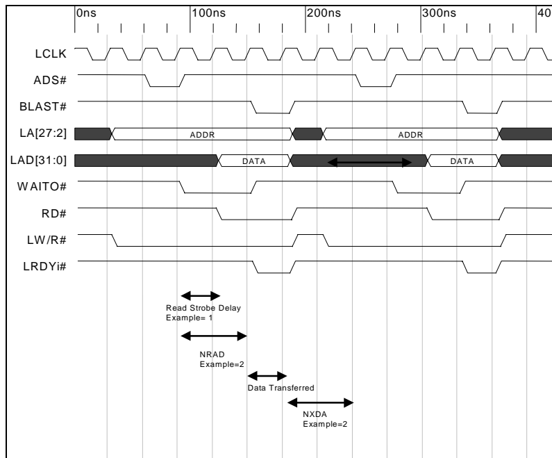
Figure 2-2. PCI 9052 Single Cycle Read
