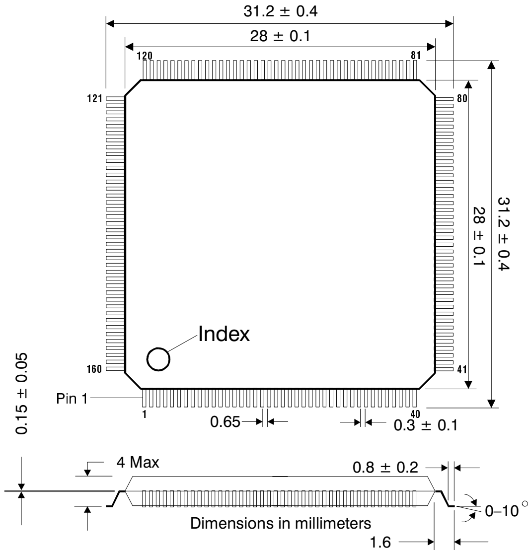
Figure 8-1. Package Mechanical Dimensions
