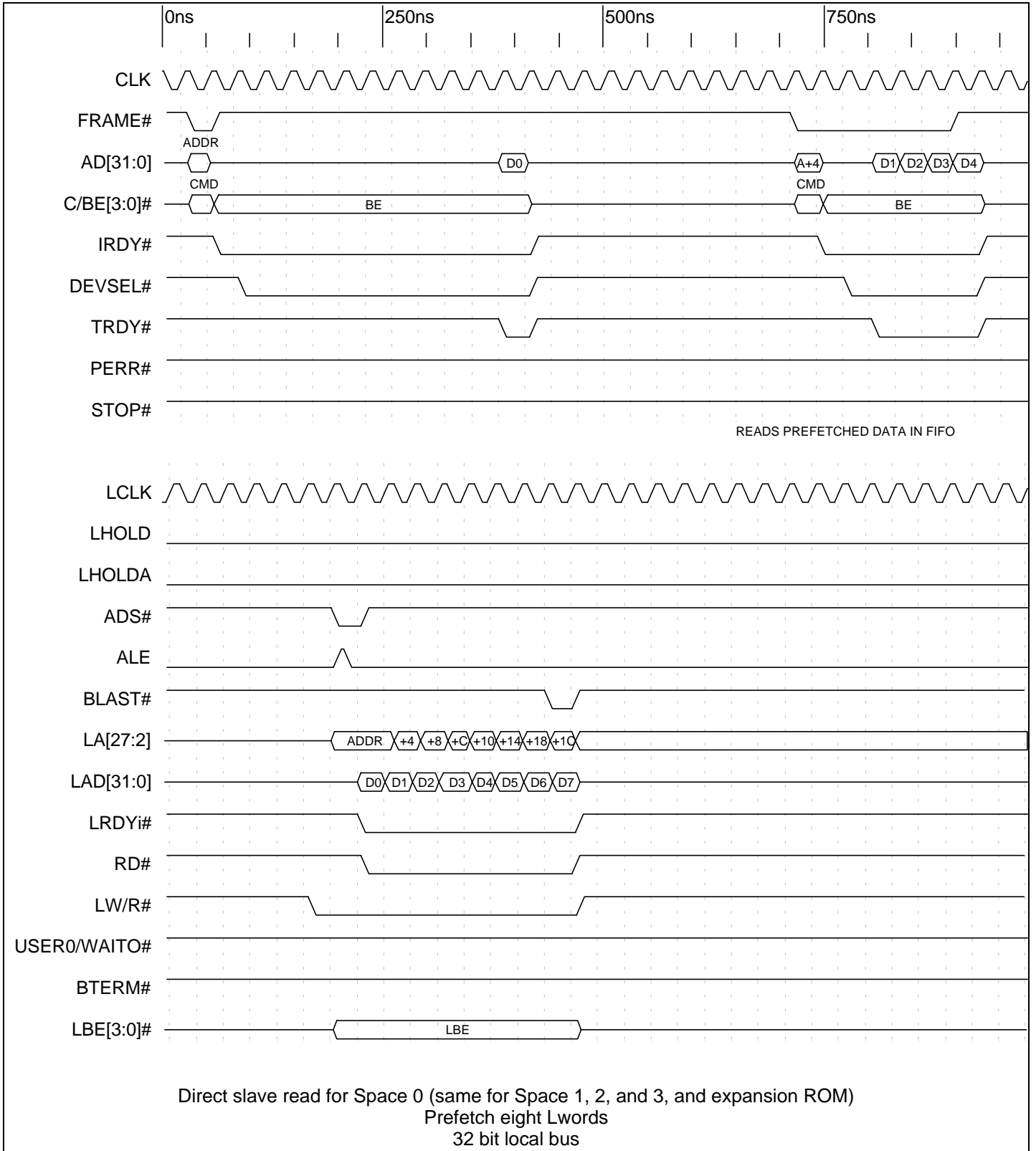
Timing Diagram 9-28. Direct Slave Read with Read Ahead Mode Enabled
